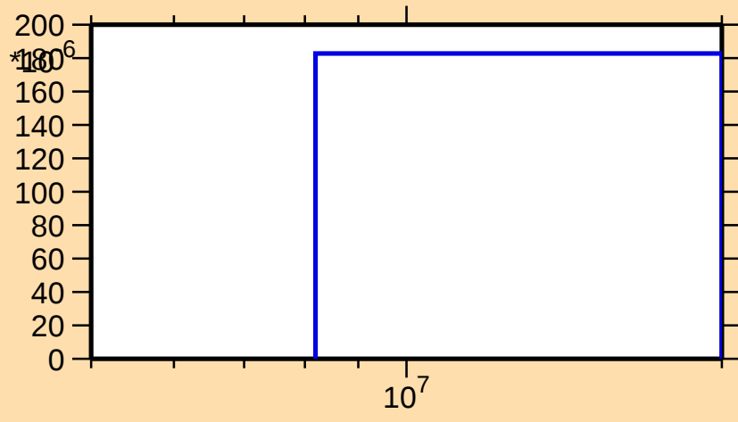
\sigma vs. E for ^{115}\text{Ag}(n,np)
