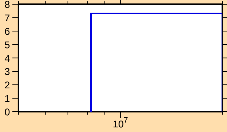
\Delta\sigma/\sigma vs. E for ^{115}\text{Ag}(n,\text{el.})
