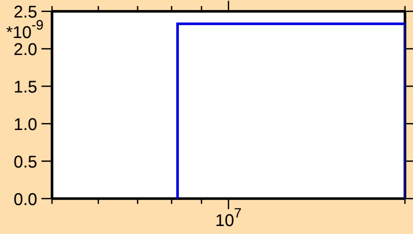
\sigma vs. E for ^{115}\text{Ag}(n,nt)
