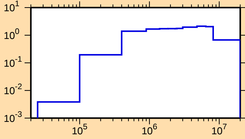
\sigma vs. E for ^{115}\text{Ag}(n,\text{inel.})
