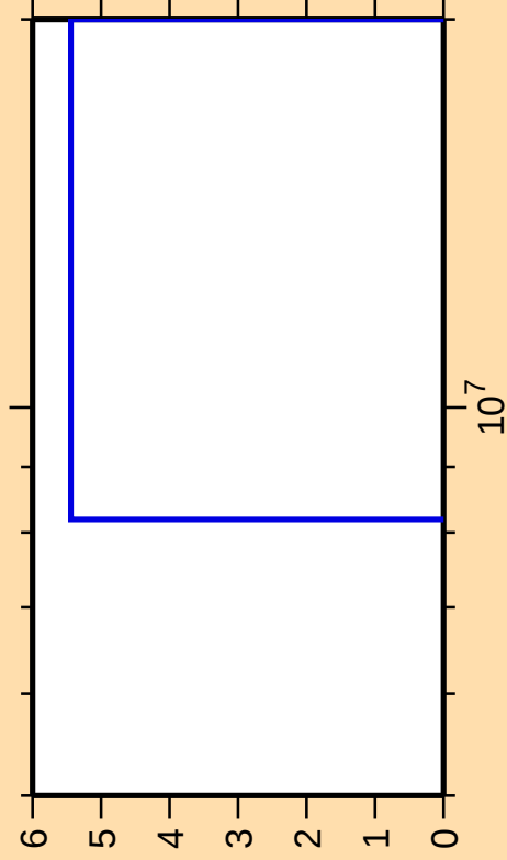
\Delta\sigma/\sigma vs. E for ^{115}\text{Ag}(n,2np)
