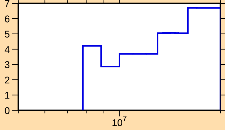
\Delta\sigma/\sigma vs. E for ^{115}\text{Ag}(n,\text{tot.})
