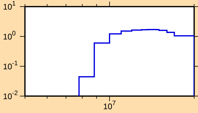
\sigma vs. E for ^{115}\text{Ag}(n,2n)
