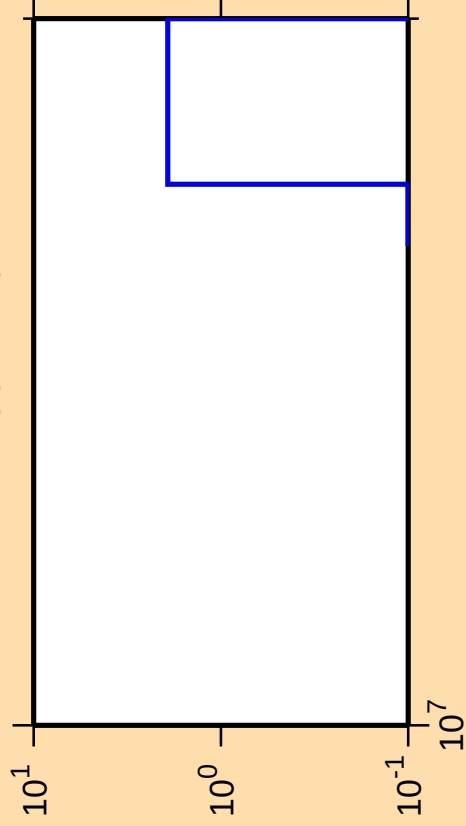
\Delta\sigma/\sigma vs. E for ^{117}\text{Ag}(n,2n\alpha)
