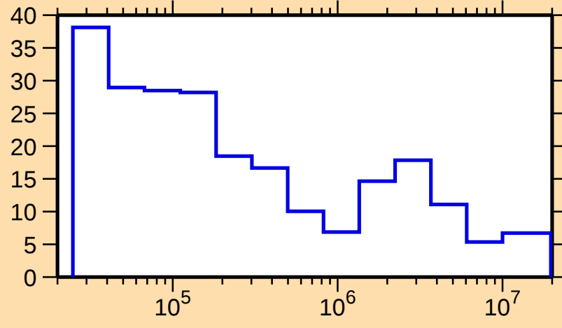
\Delta\sigma/\sigma vs. E for ^{117}\text{Ag}(\text{n,tot.})
