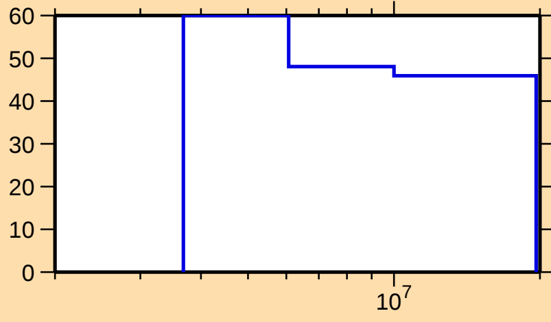
\Delta\sigma/\sigma vs. E for ^{117}\text{Ag}(n,n_1)
