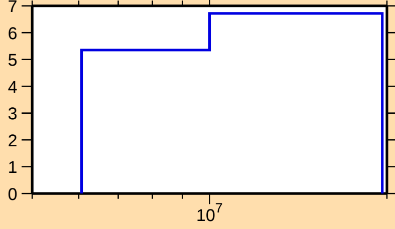
\Delta\sigma/\sigma vs. E for ^{117}\text{Ag}(n,\text{tot.})
