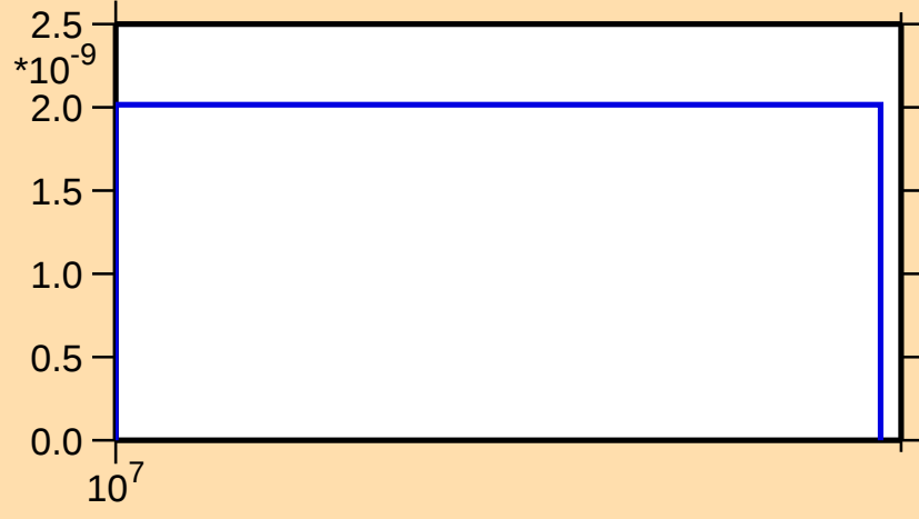
\sigma vs. E for ^{117}\text{Ag}(n,\text{nt})
