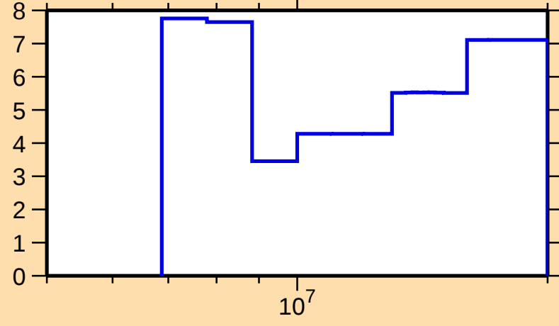
\Delta\sigma/\sigma vs. E for ^{29}\text{Al}(n,p)
