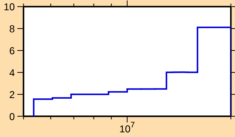
\Delta\sigma/\sigma vs. E for ^{29}\text{Al}(\text{n},\text{inel.})
