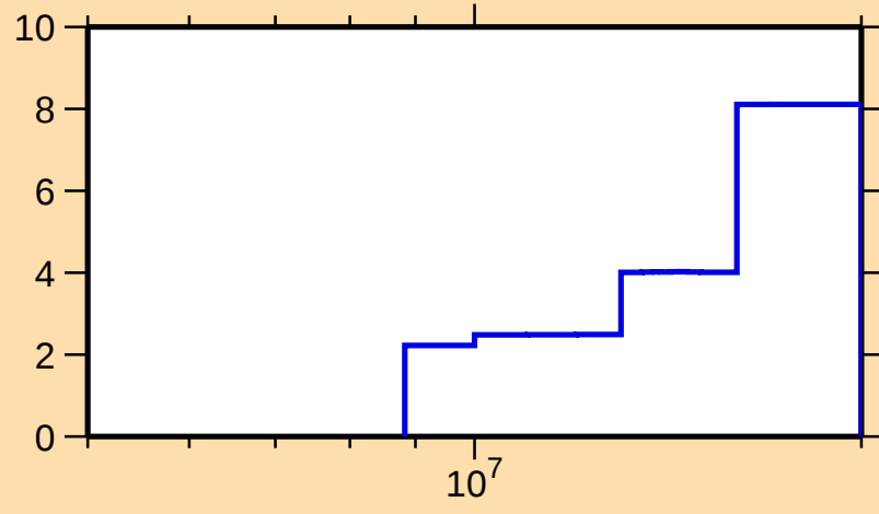
\Delta\sigma/\sigma vs. E for ^{29}\text{Al}(n,\text{inel.})
