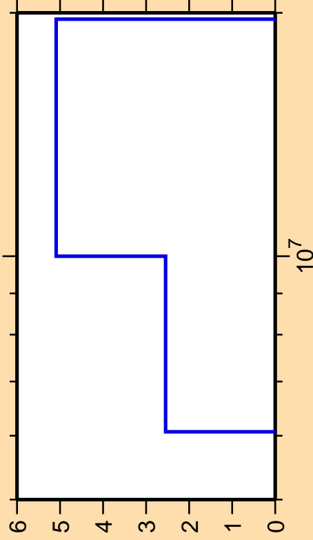
\Delta\sigma/\sigma vs. E for ^{29}\text{Al}(n,p)
