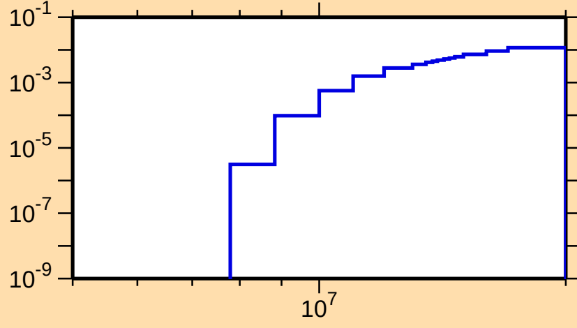
\sigma vs. E for ^{43}\text{Ar}(n,p)
