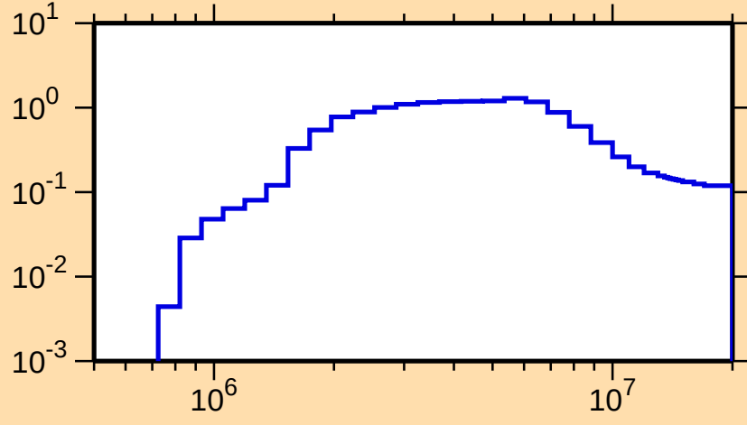
\sigma vs. E for ^{43}\text{Ar}(n,\text{inel.})
