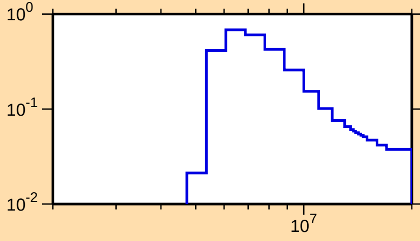
\sigma vs. E for ^{43}\text{Ar}(n,n\text{cont.})
