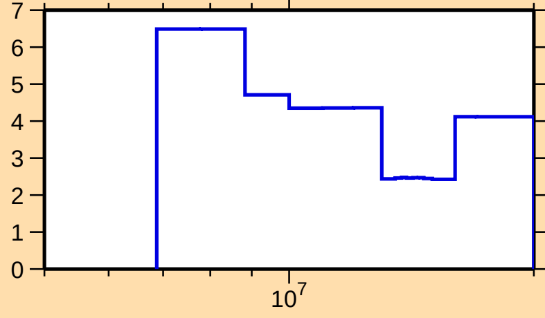
\Delta\sigma/\sigma vs. E for ^{43}\text{Ar}(n,\text{el.})
