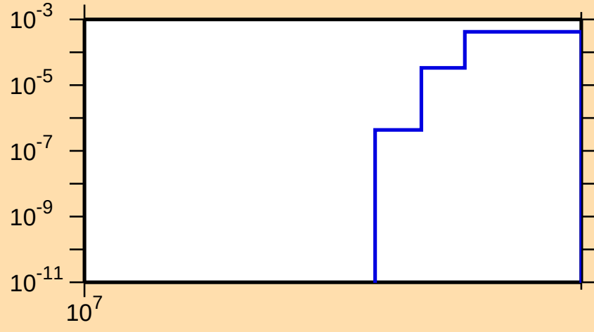
\sigma vs. E for ^{43}\text{Ar}(n,np)
