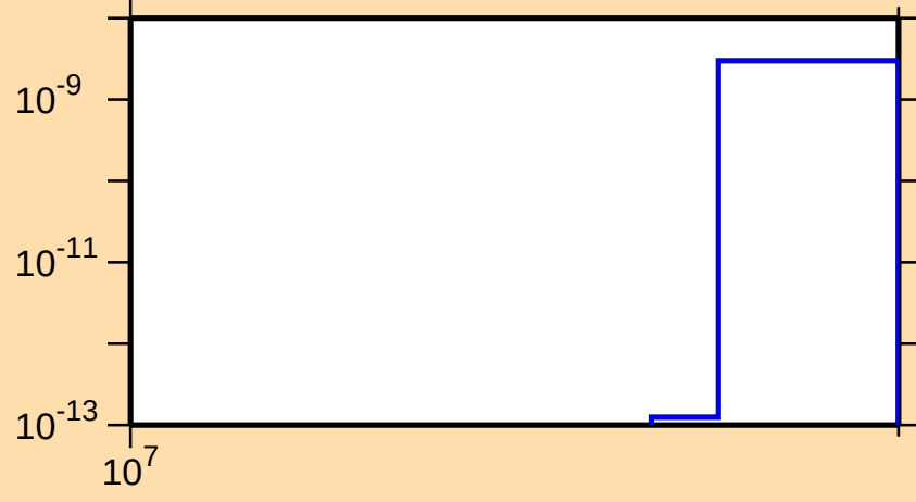
\sigma vs. E for ^{43}\text{Ar}(n,2n\alpha)
