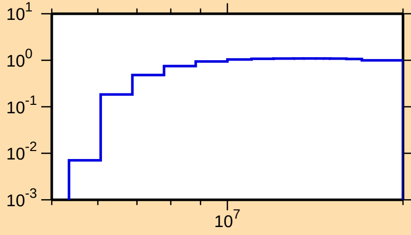
\sigma vs. E for ^{43}\text{Ar}(n,2n)
