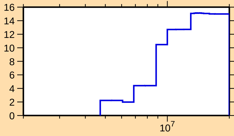
\Delta\sigma/\sigma vs. E for ^{43}\text{Ar}(n,\text{inel.})
