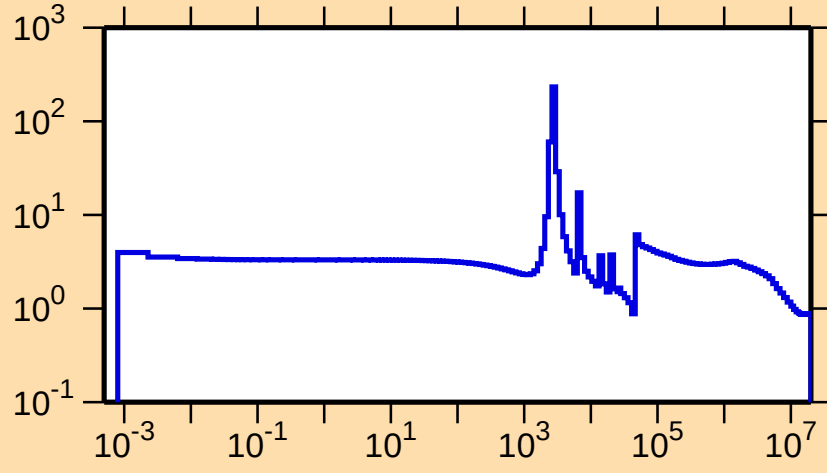
\sigma vs. E for ^{43}\text{Ar}(n,\text{el.})
