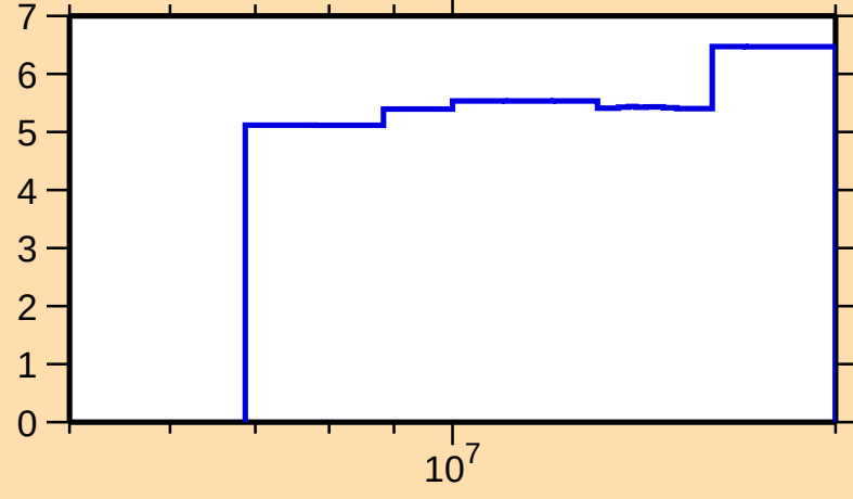
\Delta\sigma/\sigma vs. E for ^{43}\text{Ar}(n,2n)
