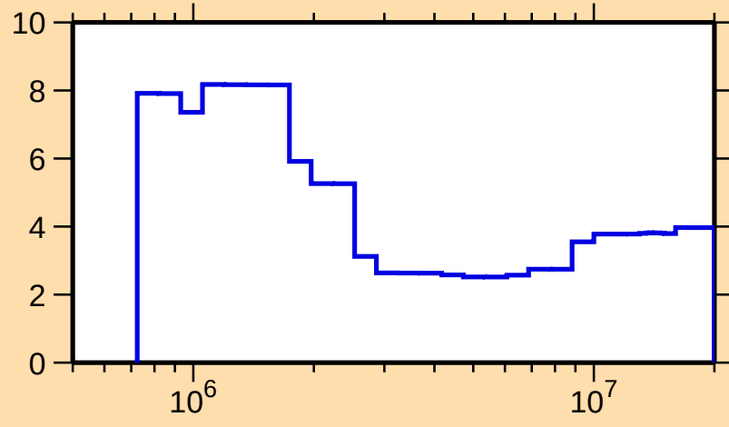
\Delta\sigma/\sigma vs. E for ^{43}\text{Ar}(n,\text{nonel.})
