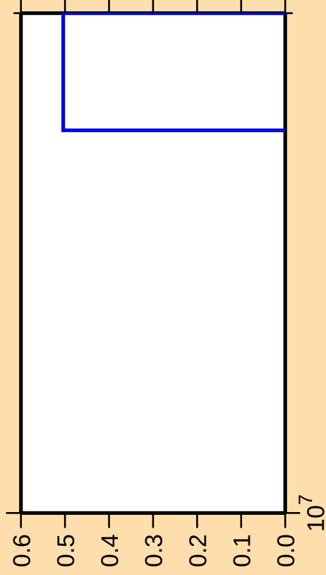
\Delta\sigma/\sigma vs. E for ^{43}\text{Ar}(n,\text{nt})
