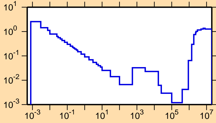
\sigma vs. E for ^{43}\text{Ar}(n,\text{nonel.})
