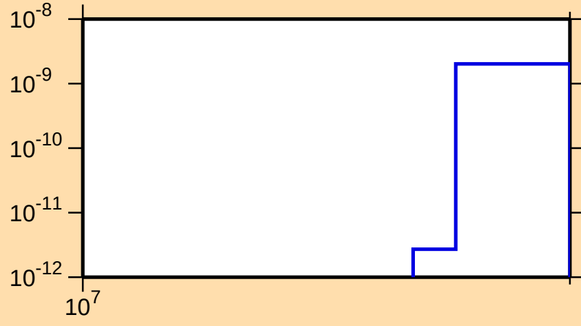
\sigma vs. E for ^{68}\text{As}(n,2n\alpha)
