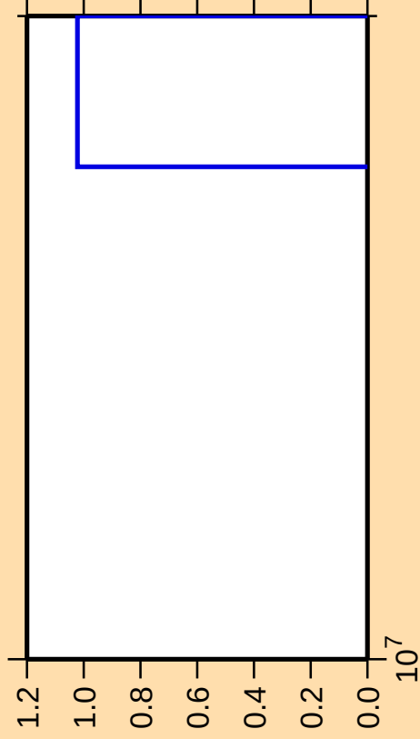
\Delta\sigma/\sigma vs. E for ^{68}\text{As}(n,nt)
