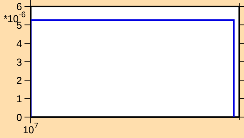
\sigma vs. E for ^{68}\text{As}(n,\text{pt})
