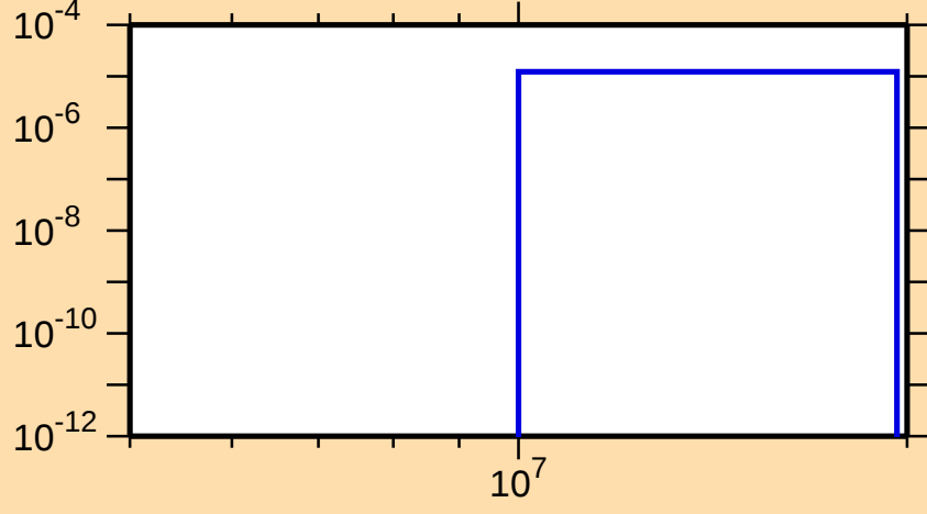
\sigma vs. E for ^{68}\text{As}(\text{mt117})
