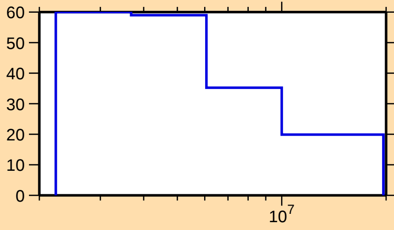
\Delta\sigma/\sigma vs. E for ^{68}\text{As}(n,n\text{cont.})
