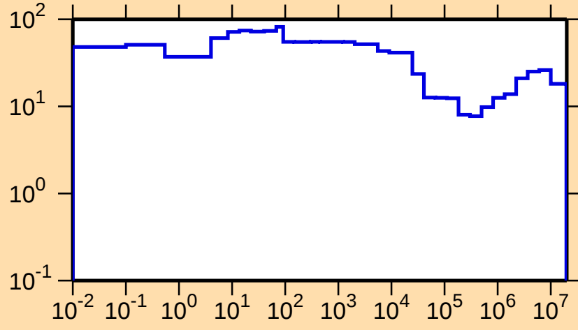
\Delta\sigma/\sigma vs. E for ^{68}\text{As}(n,p)
