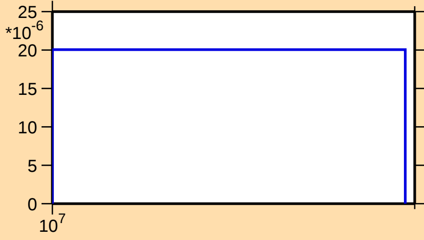
\sigma vs. E for ^{68}\text{As}(n,2np)
