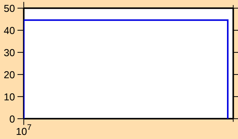
\Delta\sigma/\sigma vs. E for ^{68}\text{As}(n,2n)
