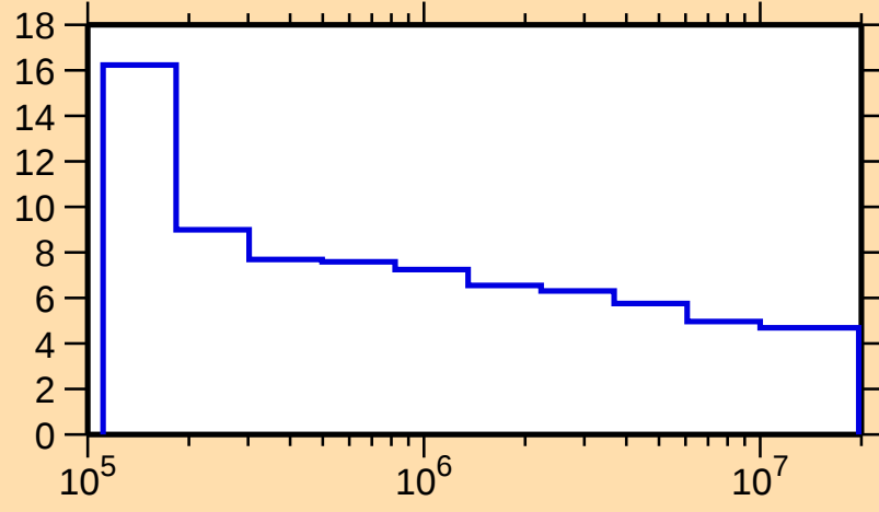
\Delta\sigma/\sigma vs. E for ^{68}\text{As}(n,\text{nonel.})
