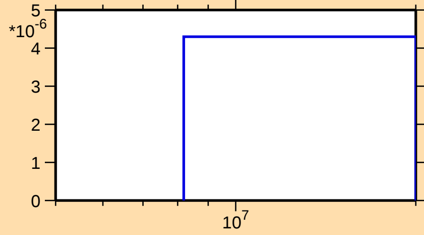
\sigma vs. E for ^{68}\text{As}(n,\text{pt})
