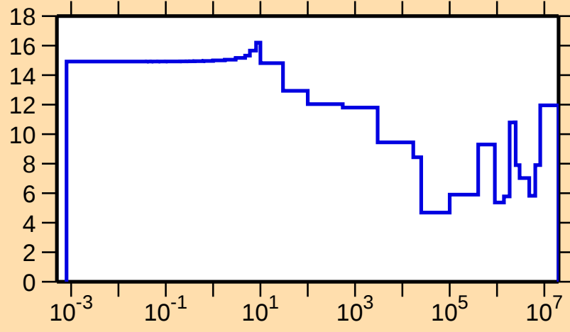
\Delta\sigma/\sigma vs. E for ^{68}\text{As}(n,\text{el.})
