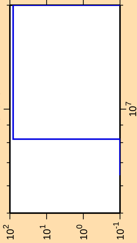
\Delta\sigma/\sigma vs. E for ^{68}\text{As}(n,\text{pd})
