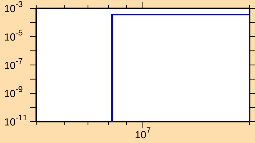
\sigma vs. E for ^{68}\text{As}(n,\text{pd})
