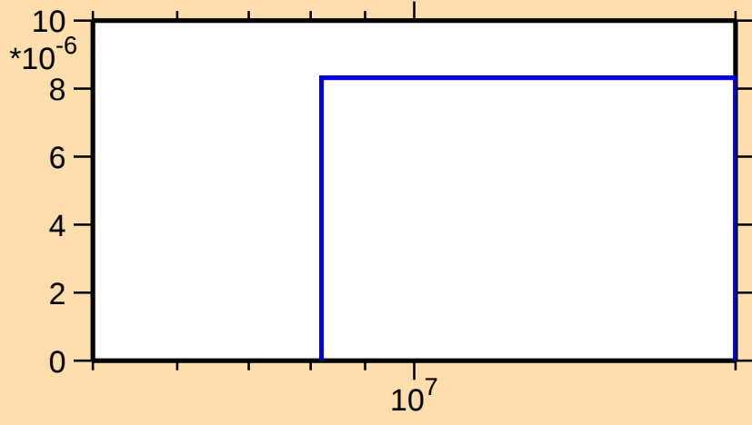
\sigma vs. E for ^{68}\text{As}(n,\text{nd})
