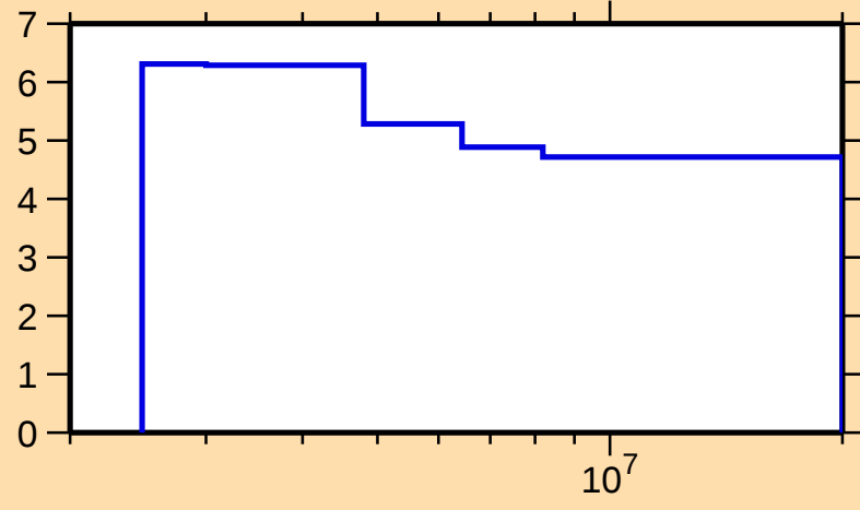
\Delta\sigma/\sigma vs. E for ^{68}\text{As}(\text{n},\text{nonel.})
