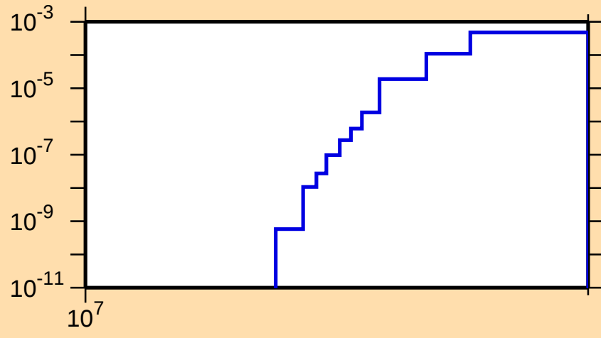
\sigma vs. E for ^{74}\text{As}(n,\text{nd})
