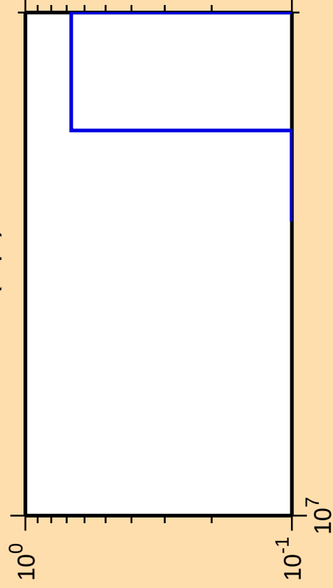
\Delta\sigma/\sigma vs. E for ^{74}\text{As}(n,\text{pt})
