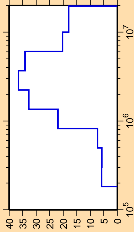
\Delta\sigma/\sigma vs. E for ^{74}\text{As}(n,n_4)
