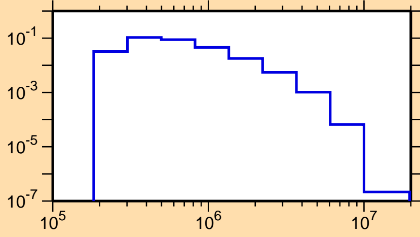
\sigma vs. E for ^{74}\text{As}(n,n_4)
