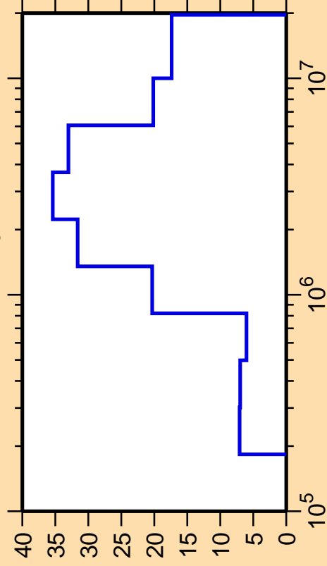
\Delta\sigma/\sigma vs. E for ^{74}\text{As}(n,n_3)
