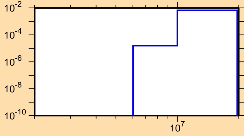
\sigma vs. E for ^{74}\text{As}(n,d)
