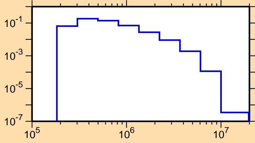
\sigma vs. E for ^{74}\text{As}(n,n_3)
