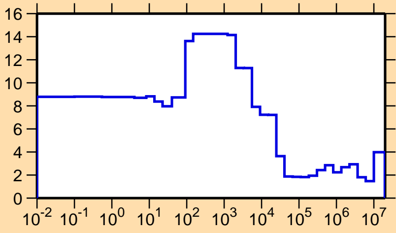
\Delta\sigma/\sigma vs. E for ^{74}\text{As}(n,el.)
