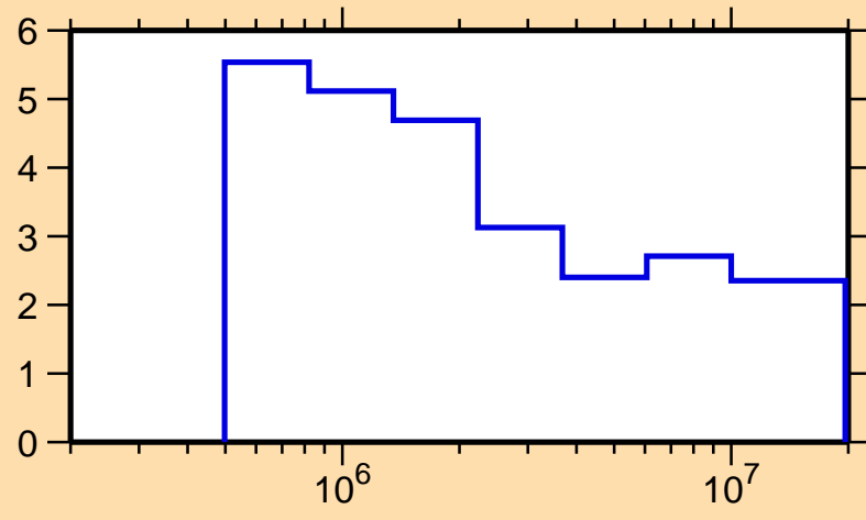
\Delta\sigma/\sigma vs. E for ^{74}\text{As}(n,n\text{onel.})
