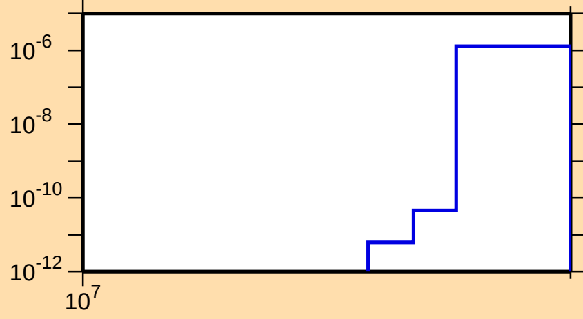
\sigma vs. E for ^{77}\text{As}(n,\text{nd})
