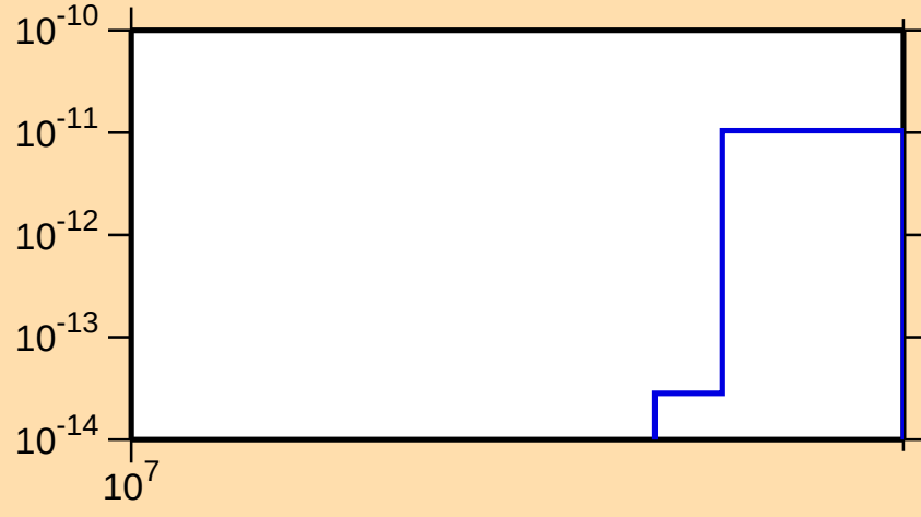
\sigma vs. E for ^{77}\text{As}(n,p\alpha)
