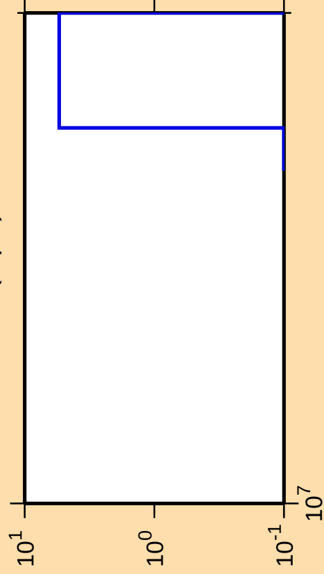
\Delta\sigma/\sigma vs. E for ^{77}\text{As}(n,p\alpha)
