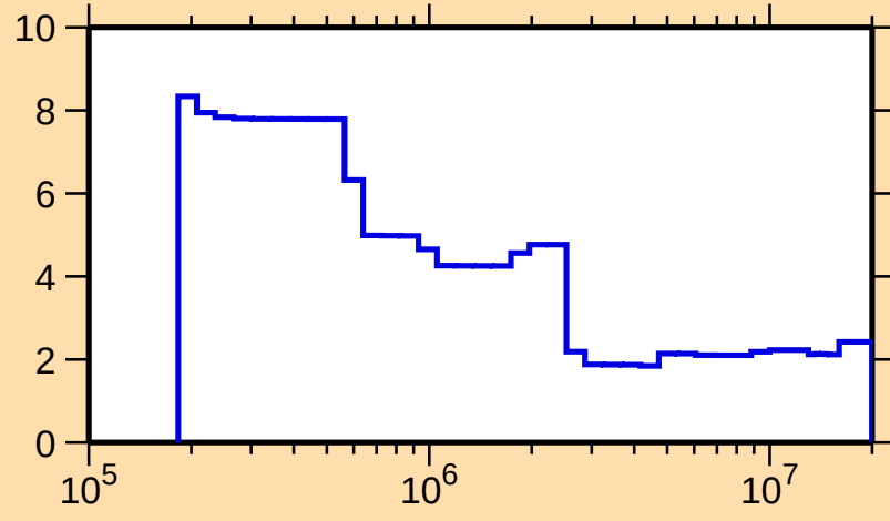
\Delta\sigma/\sigma vs. E for ^{77}\text{As}(\text{n,nonel.})
