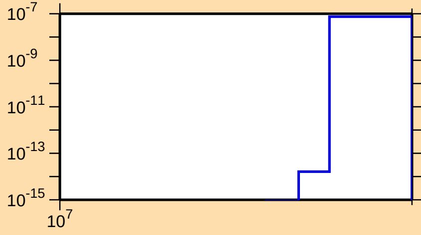
\sigma vs. E for ^{77}\text{As}(n,nt)
