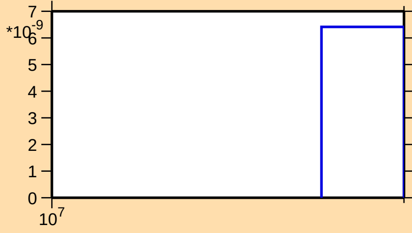
\sigma vs. E for ^{77}\text{As}(n,2np)
