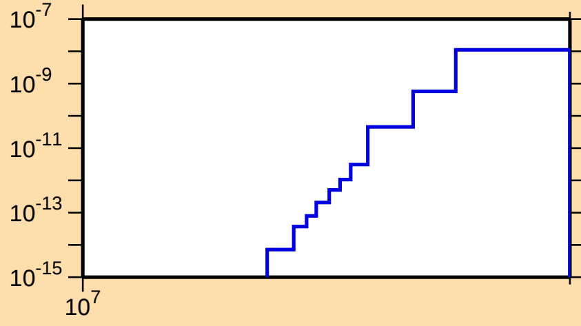
\sigma vs. E for ^{184}\text{Au}(n,\text{pt})
