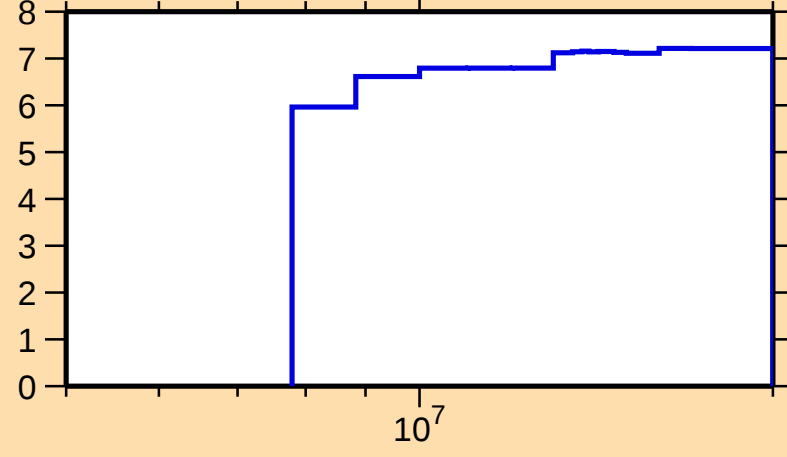
\Delta\sigma/\sigma vs. E for ^{184}\text{Au}(n,\text{nonel.})
