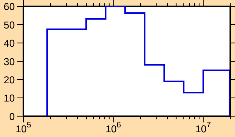
\Delta\sigma/\sigma vs. E for ^{184}\text{Au}(n,n\text{cont.})
