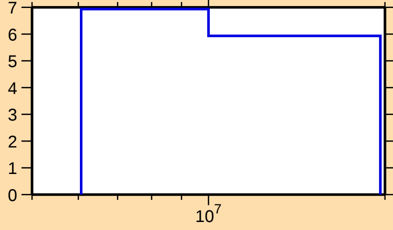
\Delta\sigma/\sigma vs. E for ^{185}\text{Au}(n,\text{nonel.})
