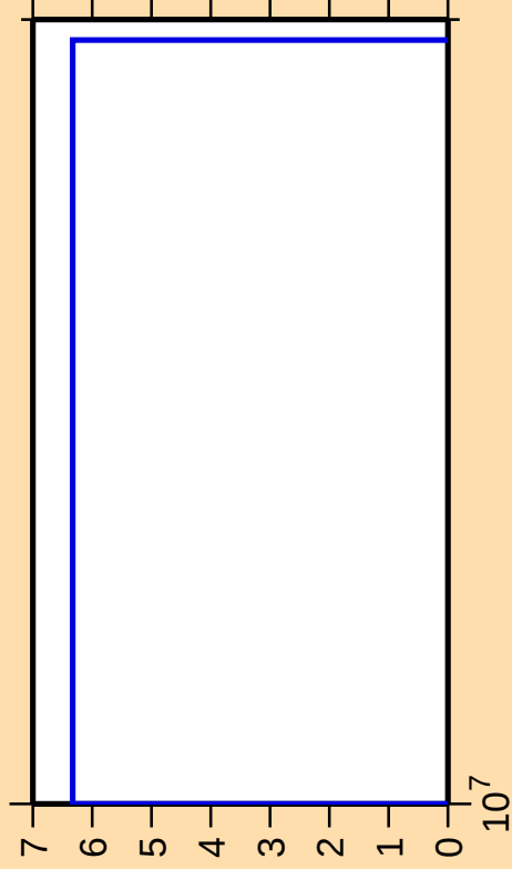
\Delta\sigma/\sigma vs. E for ^{185}\text{Au}(n,\text{pt})
