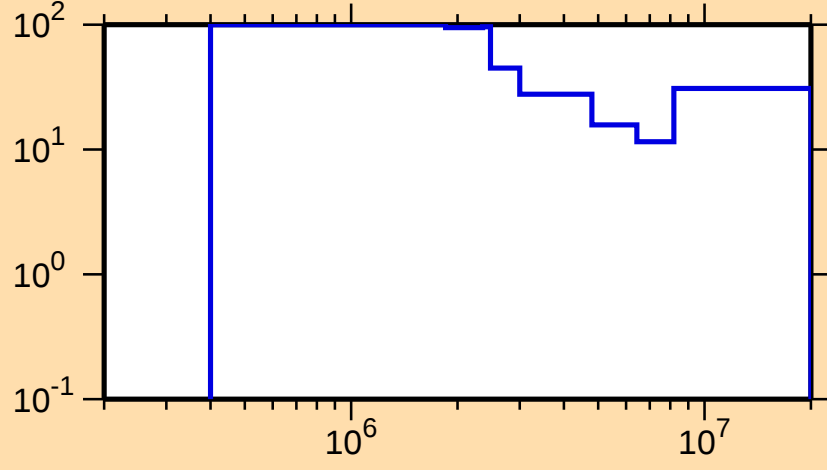
\Delta\sigma/\sigma vs. E for ^{185}\text{Au}(n,n\text{cont.})
