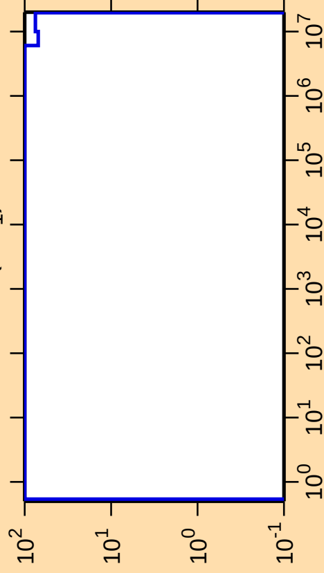
\Delta\sigma/\sigma vs. E for ^{185}\text{Au}(n,n_1)
