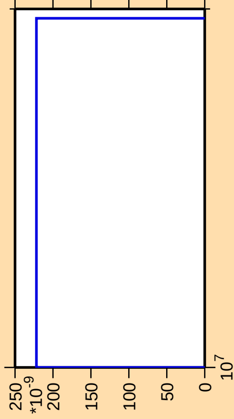
\Delta\sigma/\sigma vs. E for ^{185}\text{Au} (mt 42)
