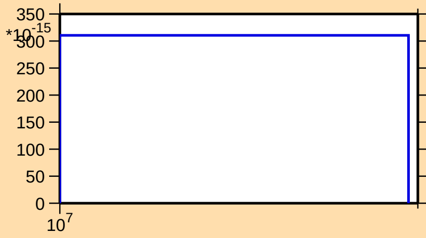
\sigma vs. E for ^{185}\text{Au}(\text{mt } 34)
