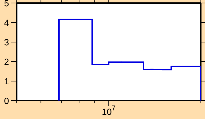
\Delta\sigma/\sigma vs. E for ^{192}\text{Au}(n,\text{tot.})
