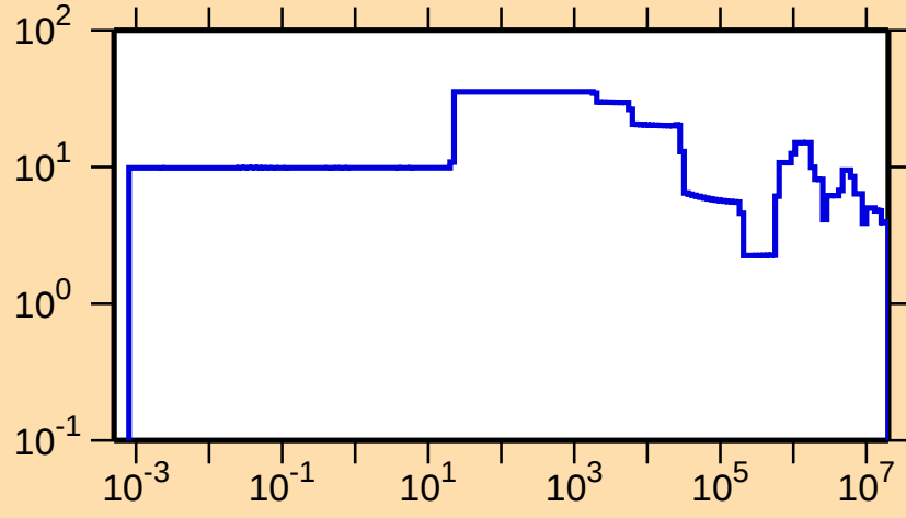
\Delta\sigma/\sigma vs. E for ^{192}\text{Au}(n,\text{el.})
