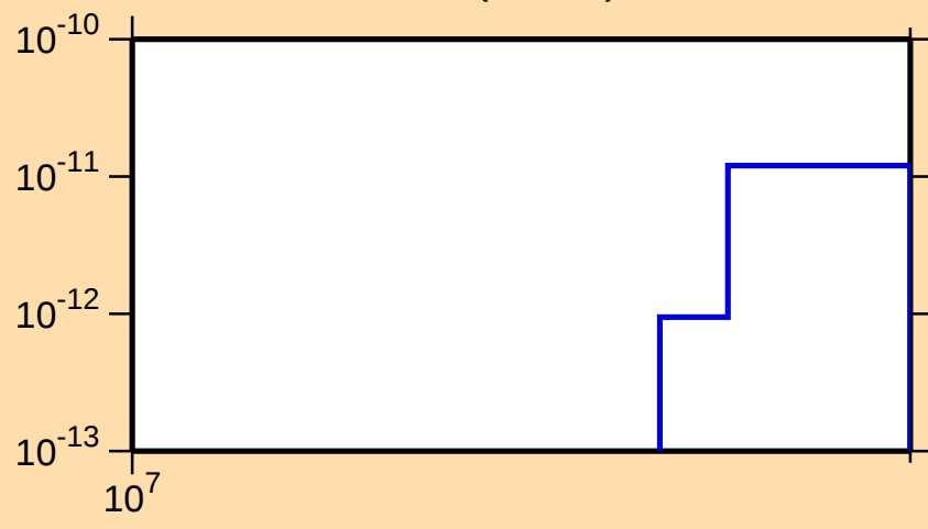
\sigma vs. E for ^{192}\text{Au}(\text{mt } 45)
