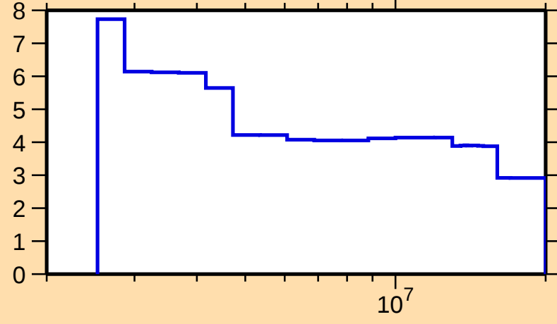
\Delta\sigma/\sigma vs. E for ^{192}\text{Au}(n,\text{nonel.})
