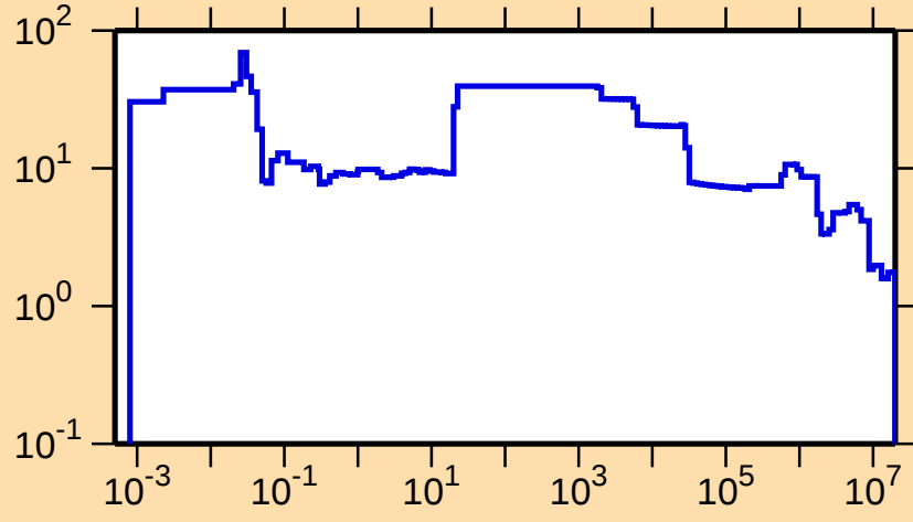
\Delta\sigma/\sigma vs. E for ^{192}\text{Au}(n,\text{tot.})
