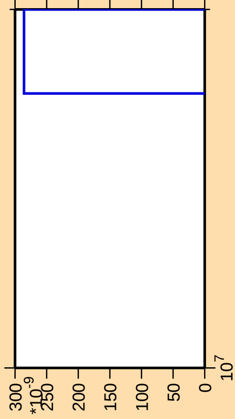
\Delta\sigma/\sigma vs. E for ^{192}\text{Au}(\text{mt } 42)
