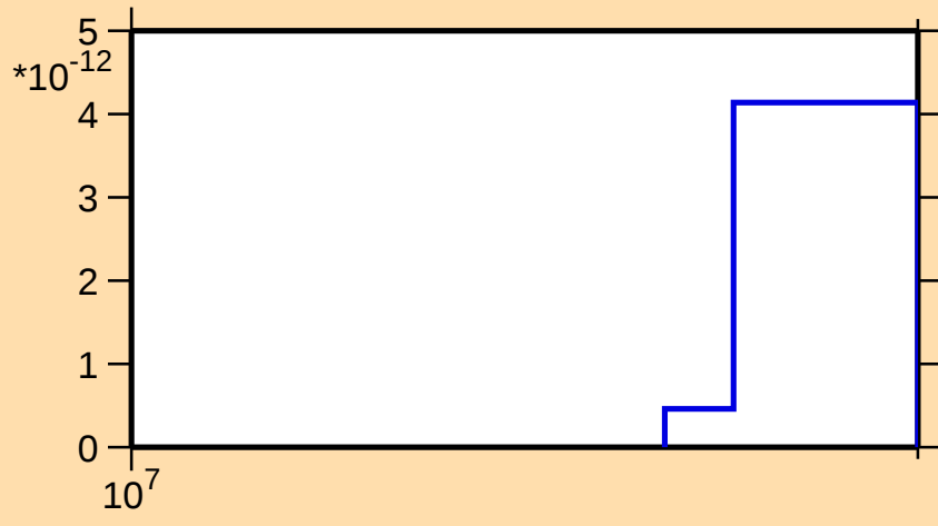
\sigma vs. E for ^{192}\text{Au}(\text{mt117})
