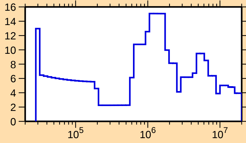
\Delta\sigma/\sigma vs. E for ^{192}\text{Au}(n,\text{el.})
