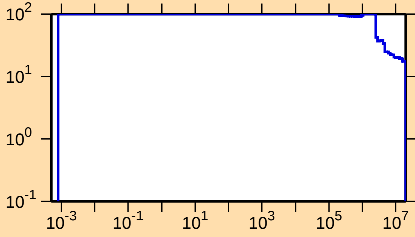
\Delta\sigma/\sigma vs. E for ^{192}\text{Au}(n,p)
