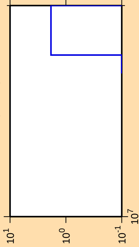
\Delta\sigma/\sigma vs. E for ^{192}\text{Au}(\text{mt } 34)
