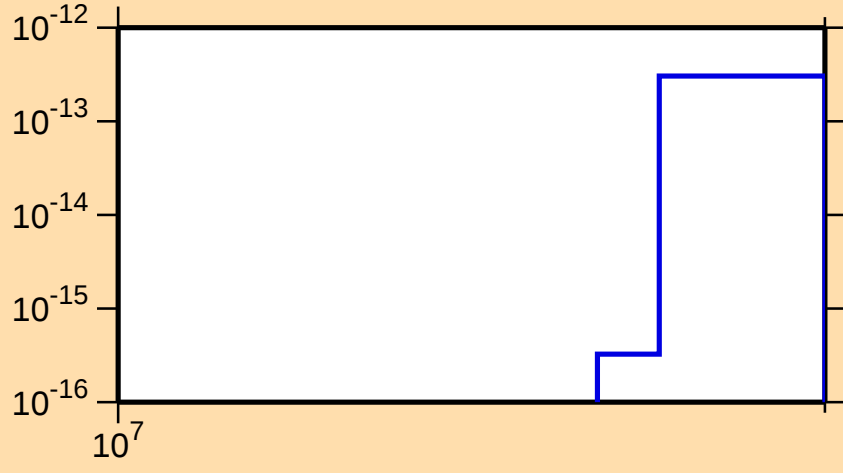
\sigma vs. E for ^{192}\text{Au}(\text{mt } 34)
