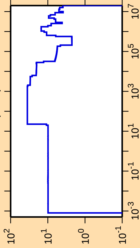
\Delta\sigma/\sigma vs. E for ^{192}\text{Au}(n,\text{el.})
