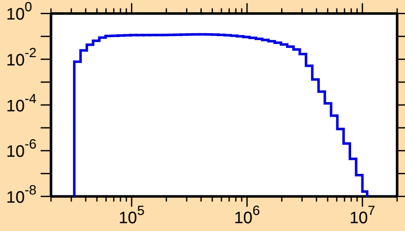
\sigma vs. E for ^{192}\text{Au}(n,n_1)
