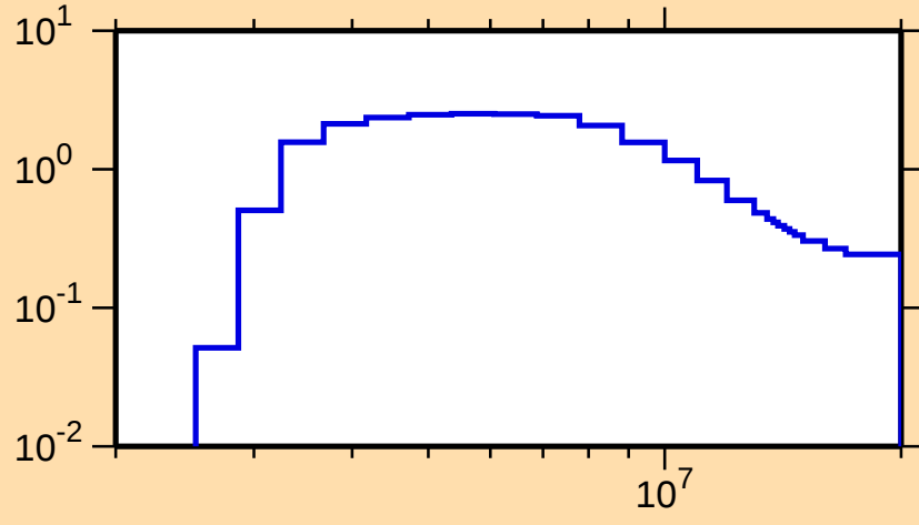
\sigma vs. E for ^{192}\text{Au}(n,n\text{cont.})
