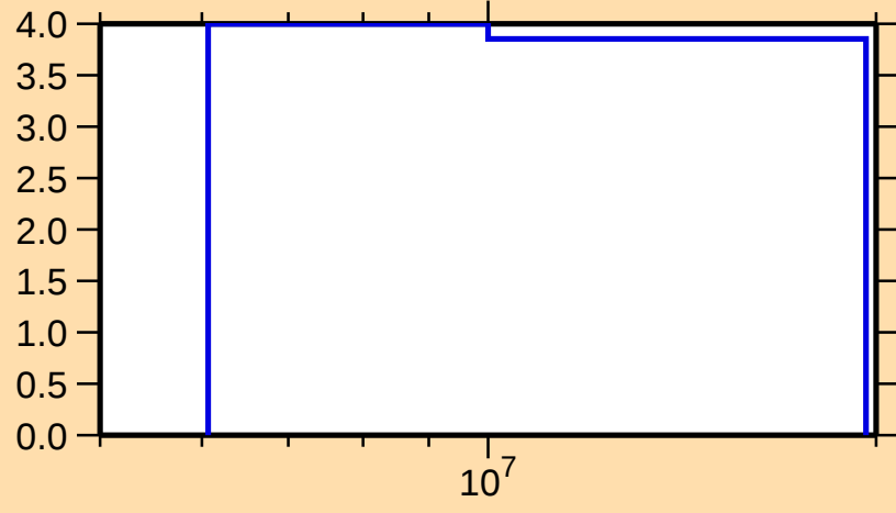
\Delta\sigma/\sigma vs. E for ^{192}\text{Au}(n,\text{nonel.})
