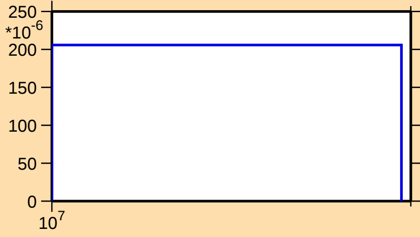
\sigma vs. E for ^{192}\text{Au}(n,3n)
