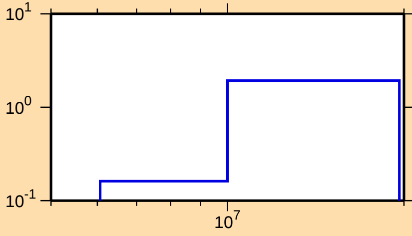
\sigma vs. E for ^{192}\text{Au}(n,2n)
