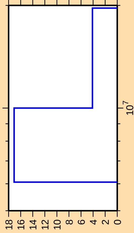
\Delta\sigma/\sigma vs. E for ^{192}\text{Au}(n,2n)
