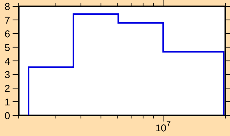
\Delta\sigma/\sigma vs. E for ^{192}\text{Au}(n,\text{el.})
