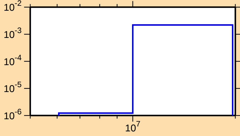
\sigma vs. E for ^{192}\text{Au}(n,np)
