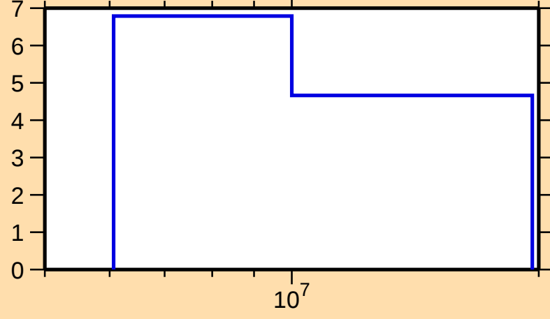
\Delta\sigma/\sigma vs. E for ^{192}\text{Au}(n,\text{el.})
