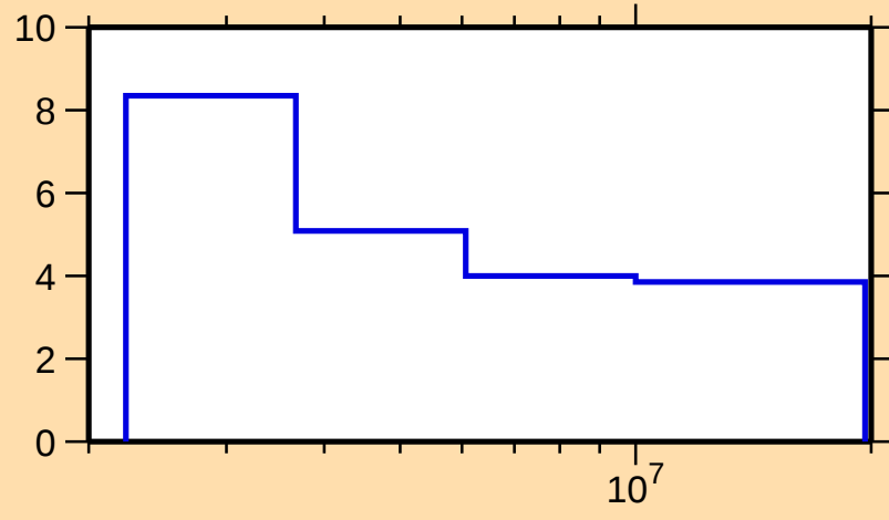
\Delta\sigma/\sigma vs. E for ^{192}\text{Au}(n,\text{nonel.})
