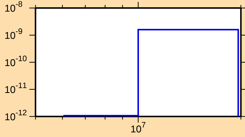
\sigma vs. E for ^{192}\text{Au}(n,p\alpha)
