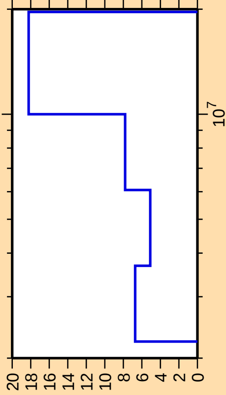
\Delta\sigma/\sigma vs. E for ^{192}\text{Au}(n,n\text{cont.})
