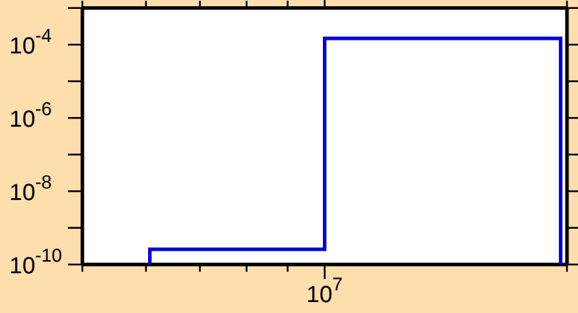
\sigma vs. E for ^{192}\text{Au}(n,t)
