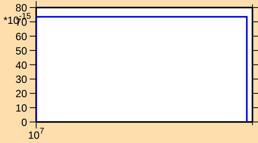
\sigma vs. E for ^{192}\text{Au}(\text{mt117})
