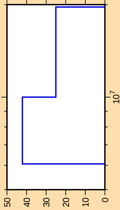
\Delta\sigma/\sigma vs. E for ^{192}\text{Au}(n,np)
