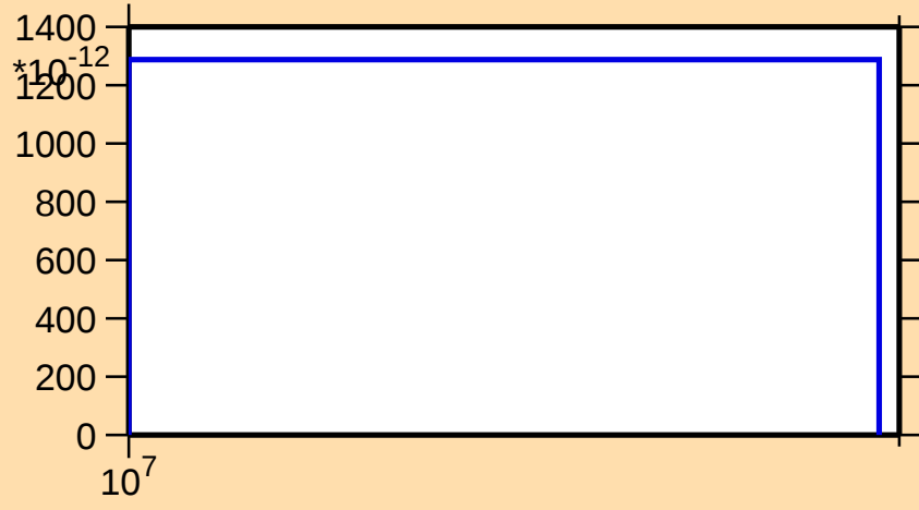
\sigma vs. E for ^{192}\text{Au}(n,\text{He}3)
