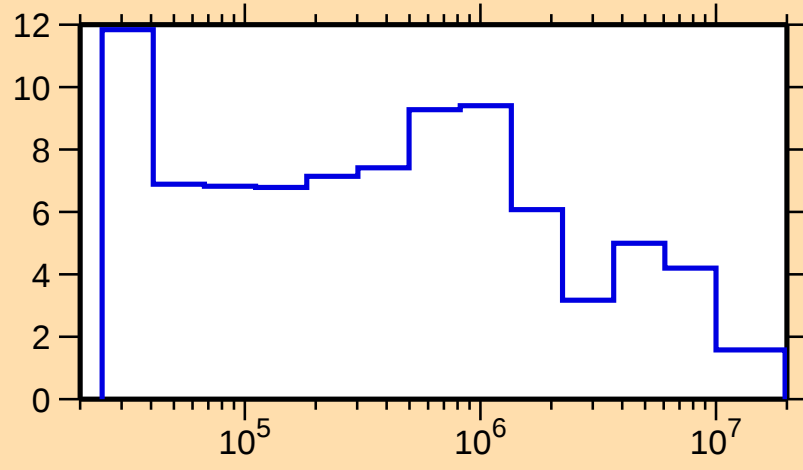
\Delta\sigma/\sigma vs. E for ^{192}\text{Au}(n,\text{tot.})
