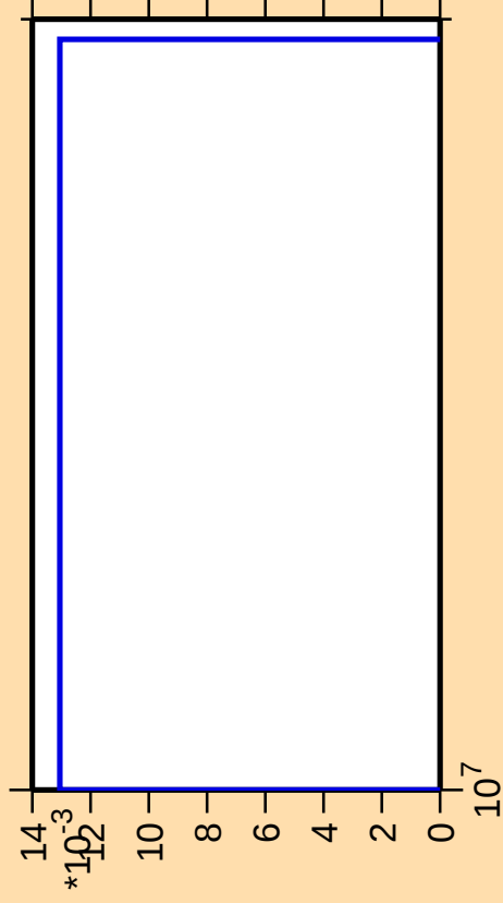
\Delta\sigma/\sigma vs. E for ^{192}\text{Au}(\text{mt } 34)
