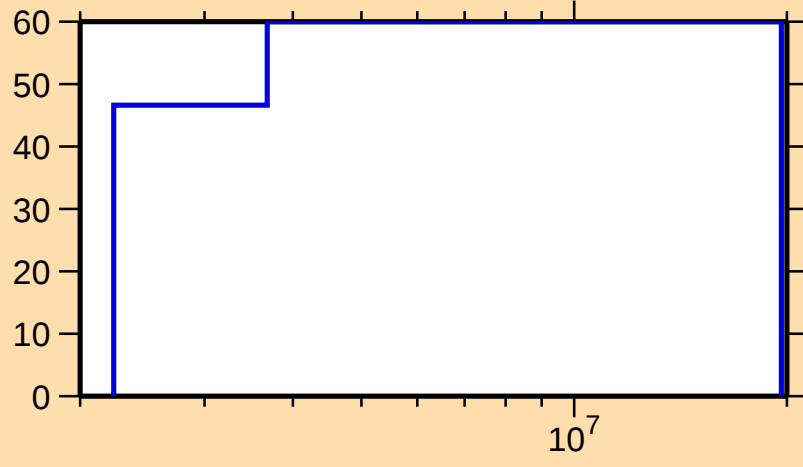
\Delta\sigma/\sigma vs. E for ^{192}\text{Au}(n,n_1)
