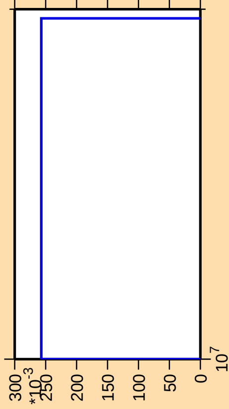
\Delta\sigma/\sigma vs. E for ^{192}\text{Au}(\text{mt117})
