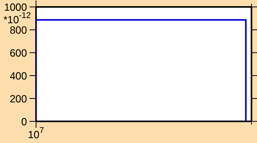
\sigma vs. E for ^{192}\text{Au}(n,nt)
