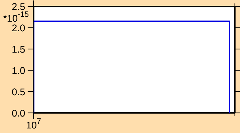
\sigma vs. E for ^{192}\text{Au}(\text{mt } 34)
