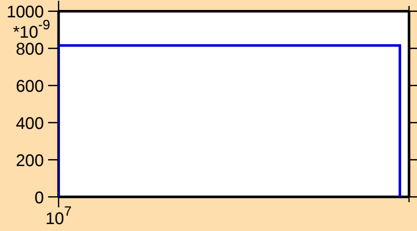
\sigma vs. E for ^{192}\text{Au}(n,2np)
