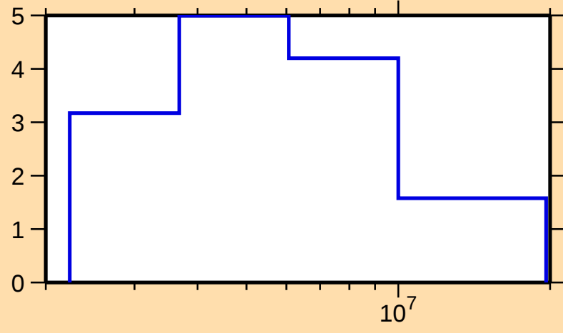
\Delta\sigma/\sigma vs. E for ^{192}\text{Au}(n,\text{tot.})
