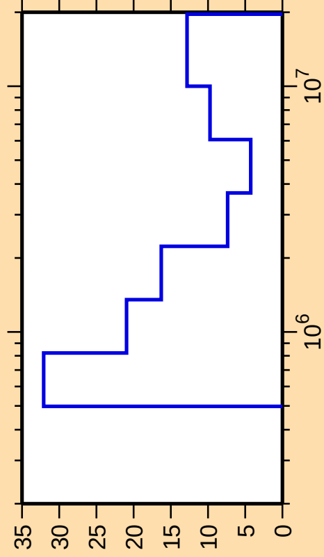
\Delta\sigma/\sigma vs. E for ^{196}\text{Au}(n,n\text{cont.})
