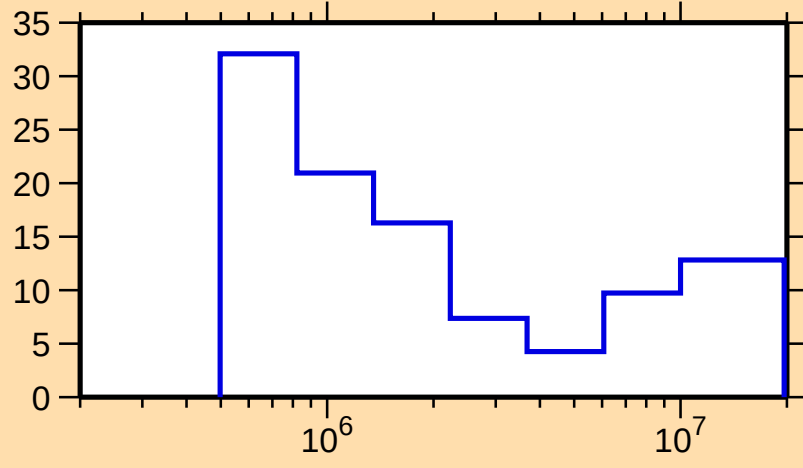
\Delta\sigma/\sigma vs. E for ^{196}\text{Au}(n,n\text{cont.})
