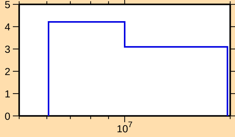
\Delta\sigma/\sigma vs. E for ^{196}\text{Au}(n,\text{el.})
