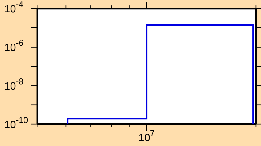
\sigma vs. E for ^{196}\text{Au}(n,n\alpha)
