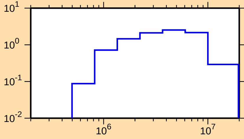
\sigma vs. E for ^{196}\text{Au}(n,n\text{cont.})
