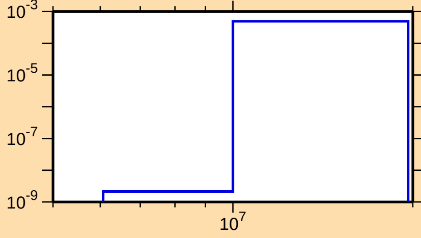
\sigma vs. E for ^{196}\text{Au}(n,np)
