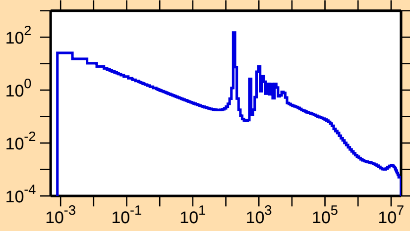
\sigma vs. E for ^{204}\text{Au}(n,\gamma)
