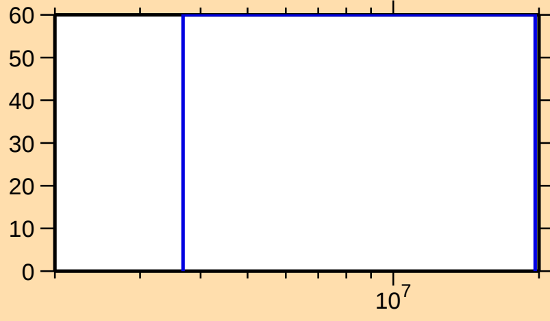
\Delta\sigma/\sigma vs. E for ^{204}\text{Au}(n,\gamma)
