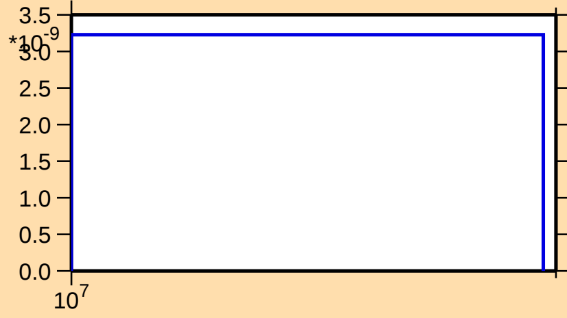
\sigma vs. E for ^{204}\text{Au}(n,\text{nd})
