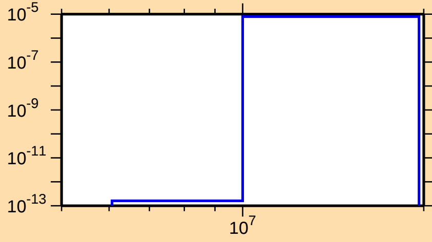
\sigma vs. E for ^{204}\text{Au}(n,t)
