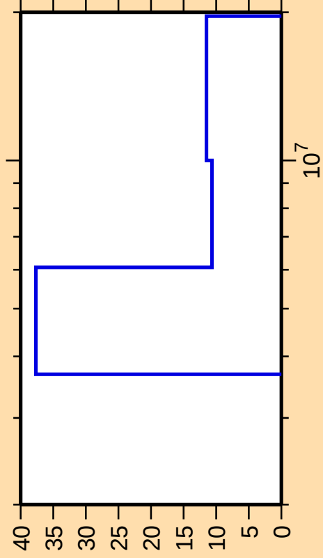
\Delta\sigma/\sigma vs. E for ^{204}\text{Au}(n,2n)
