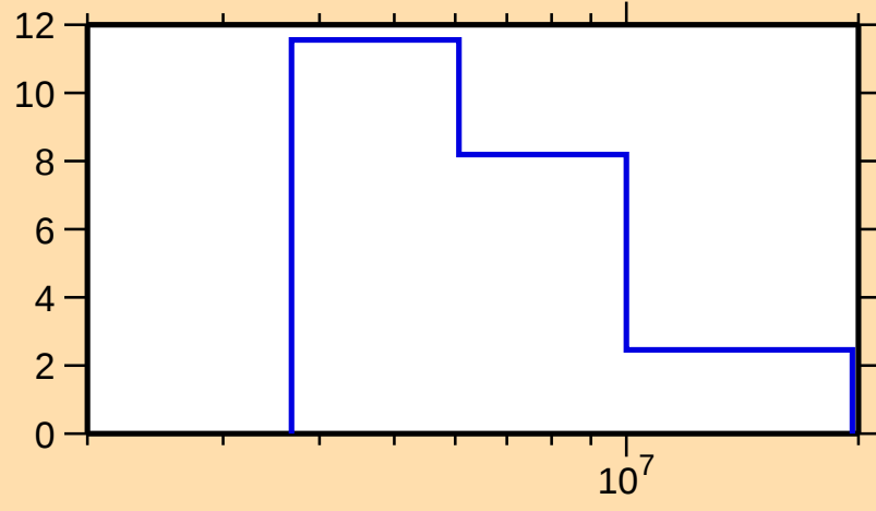
\Delta\sigma/\sigma vs. E for ^{204}\text{Au}(n,\text{tot.})
