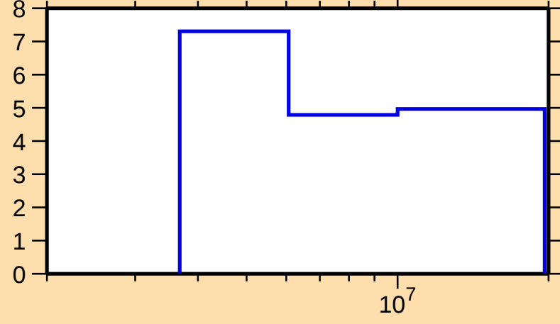
\Delta\sigma/\sigma vs. E for ^{204}\text{Au}(n,\text{nonel.})
