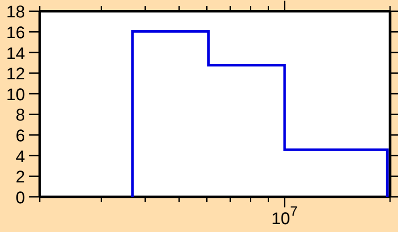
\Delta\sigma/\sigma vs. E for ^{204}\text{Au}(n,\text{el.})
