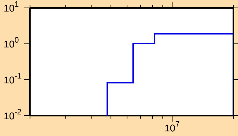
\sigma vs. E for ^{204}\text{Au}(n,2n)
