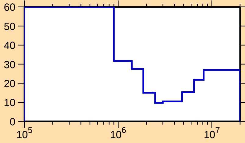
\Delta\sigma/\sigma vs. E for ^{204}\text{Au}(n,n\text{cont.})
