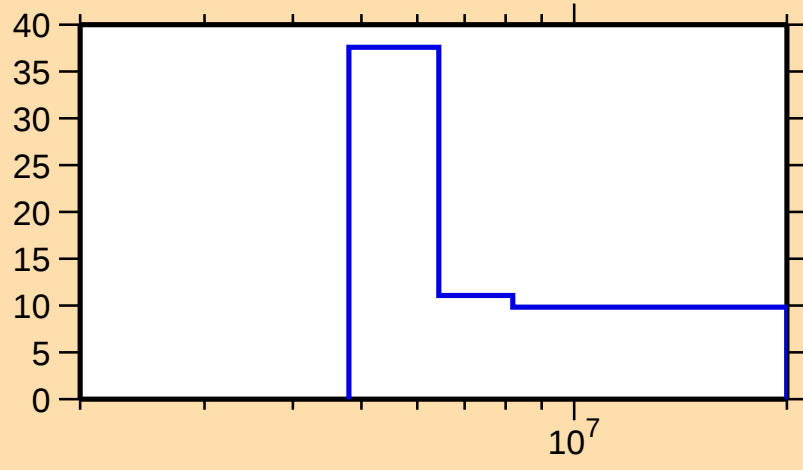
\Delta\sigma/\sigma vs. E for ^{204}\text{Au}(n,2n)
