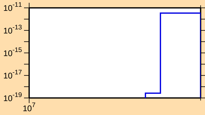
\sigma vs. E for ^{130}\text{Ba}(n,\text{nt})
