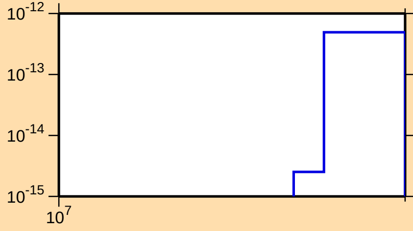
\sigma vs. E for ^{130}\text{Ba}(\text{mt117})
