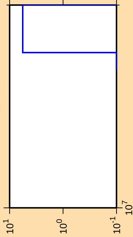
\Delta\sigma/\sigma vs. E for ^{130}\text{Ba}(n,\text{nt})
