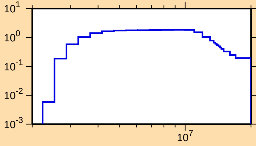
\sigma vs. E for ^{130}\text{Ba}(n,n\text{cont.})
