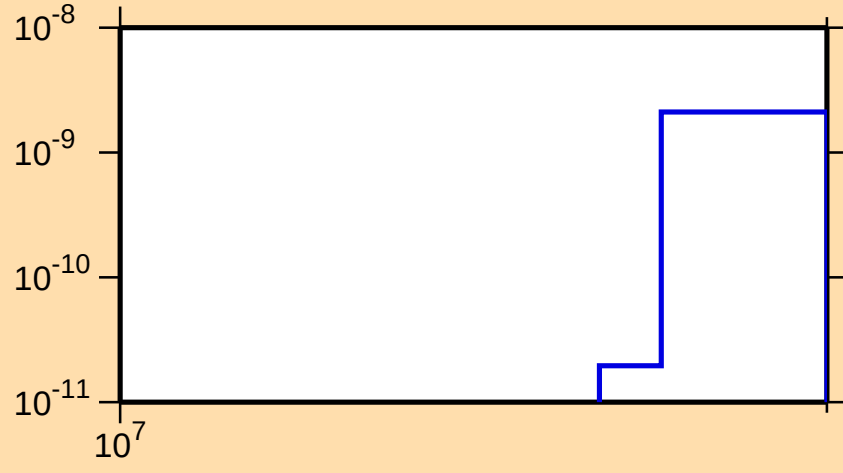
\sigma vs. E for ^{130}\text{Ba}(n,\text{pd})
