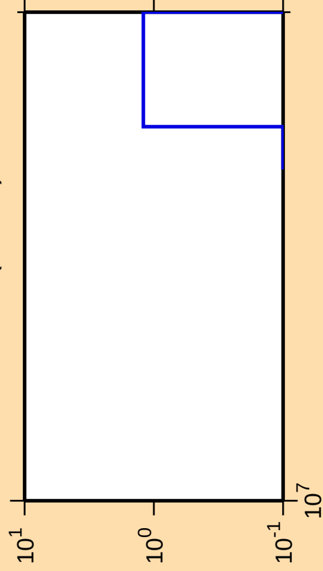
\Delta\sigma/\sigma vs. E for ^{130}\text{Ba}(\text{mt117})
