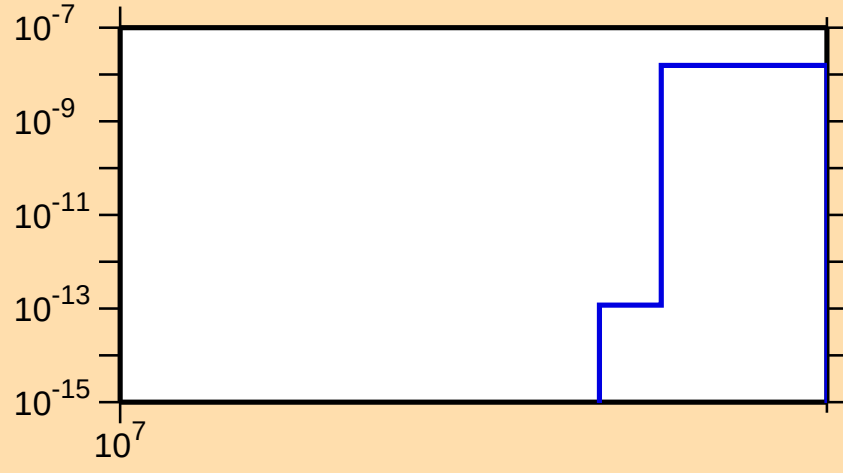
\sigma vs. E for ^{130}\text{Ba}(n,\text{nd})
