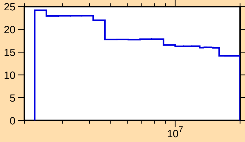
\Delta\sigma/\sigma vs. E for ^{130}\text{Ba}(n,n_1)
