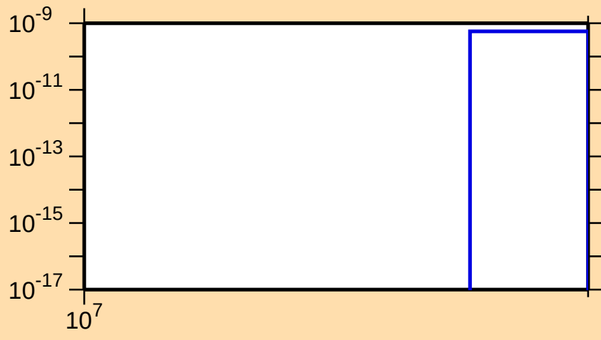
\sigma vs. E for ^{130}\text{Ba}(n,2np)
