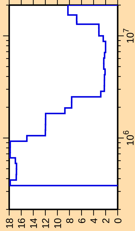
\Delta\sigma/\sigma vs. E for ^{130}\text{Ba}(n,\text{inel.})
