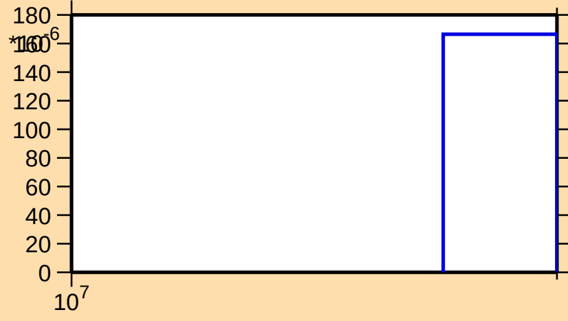
\sigma vs. E for ^{130}\text{Ba}(n,3n)
