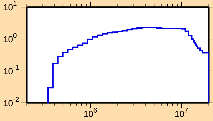
\sigma vs. E for ^{130}\text{Ba}(n,\text{inel.})
