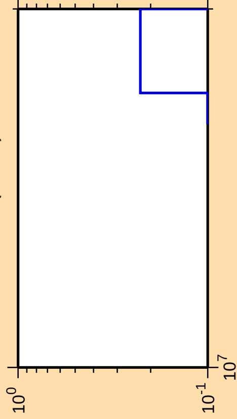
\Delta\sigma/\sigma vs. E for ^{130}\text{Ba} (mt 45)
