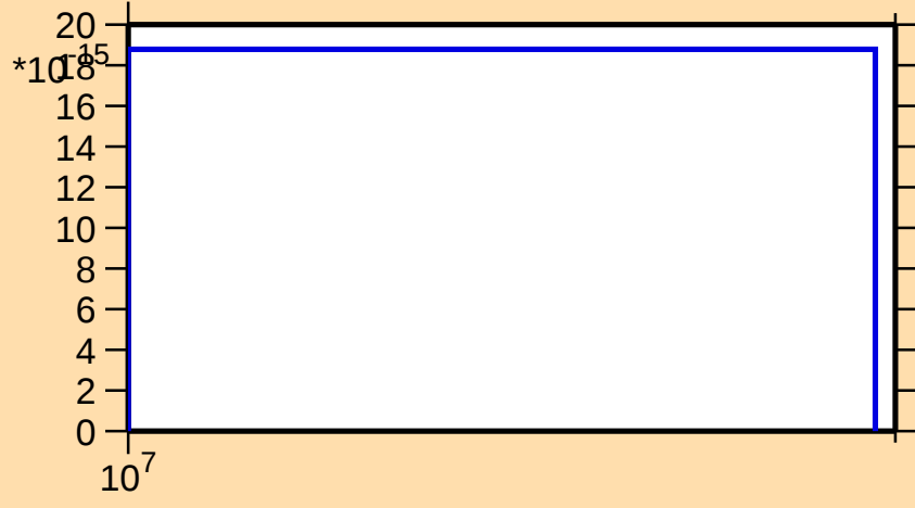
\sigma vs. E for ^{130}\text{Ba}(n,nt)
