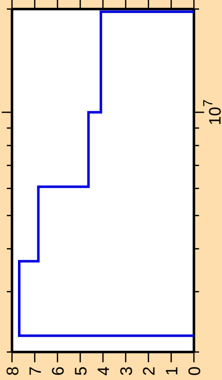
\Delta\sigma/\sigma vs. E for ^{130}\text{Ba}(n,n_{\text{cont}})
