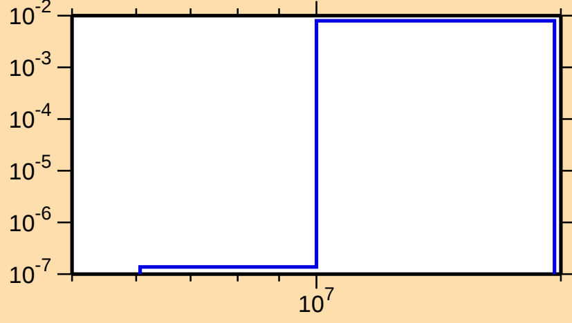
\sigma vs. E for ^{130}\text{Ba}(n,np)
