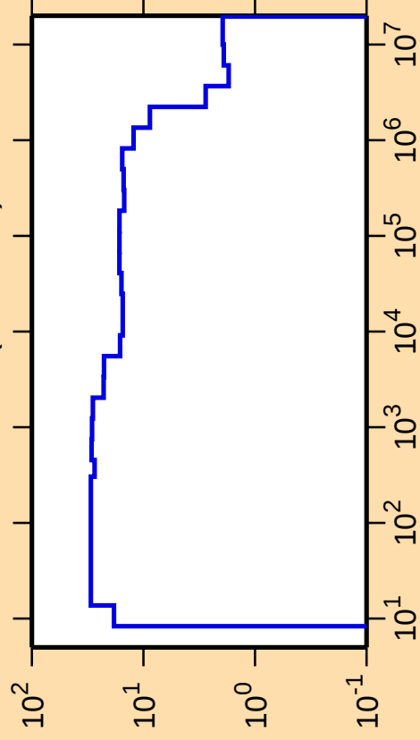
\Delta\sigma/\sigma vs. E for ^{130}\text{Ba}(n,\text{nonel.})
