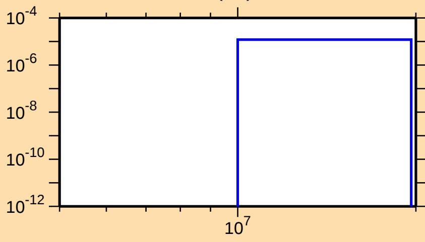
\sigma vs. E for ^{130}\text{Ba}(n,t)
