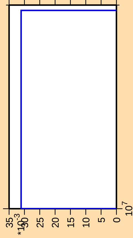
\Delta\sigma/\sigma vs. E for ^{130}\text{Ba}(n,nt)
