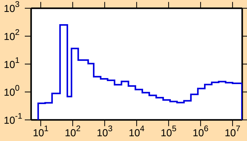
\sigma vs. E for ^{130}\text{Ba}(n,\text{nonel.})
