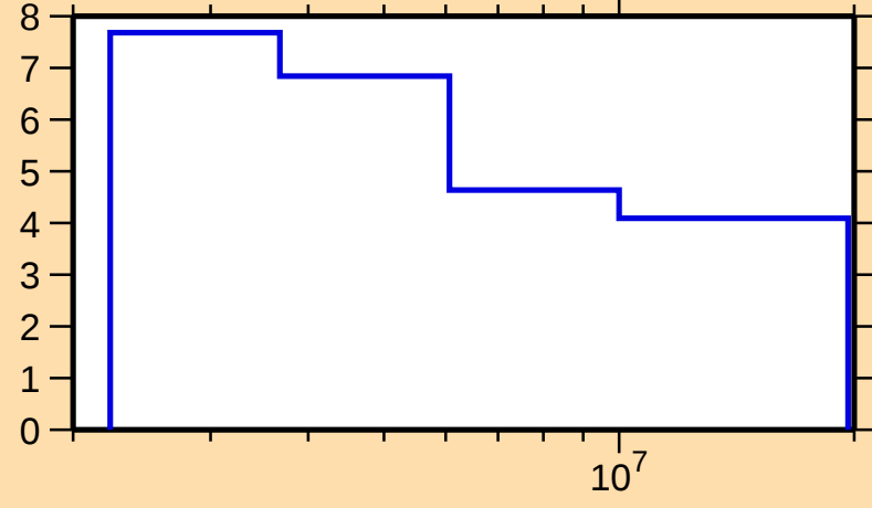
\Delta\sigma/\sigma vs. E for ^{130}\text{Ba}(n,n\text{cont.})
