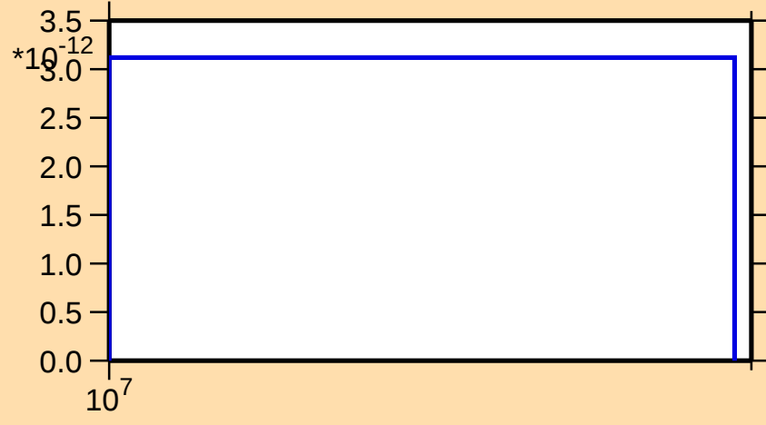
\sigma vs. E for ^{130}\text{Ba}(n,2np)
