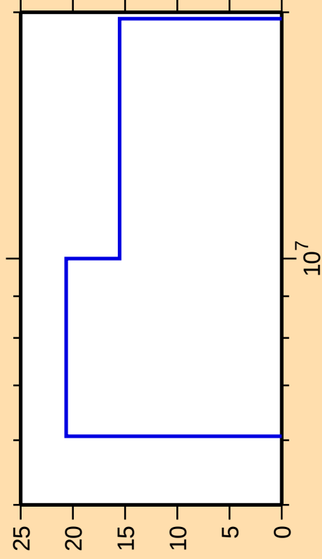
\Delta\sigma/\sigma vs. E for ^{130}\text{Ba}(n,np)
