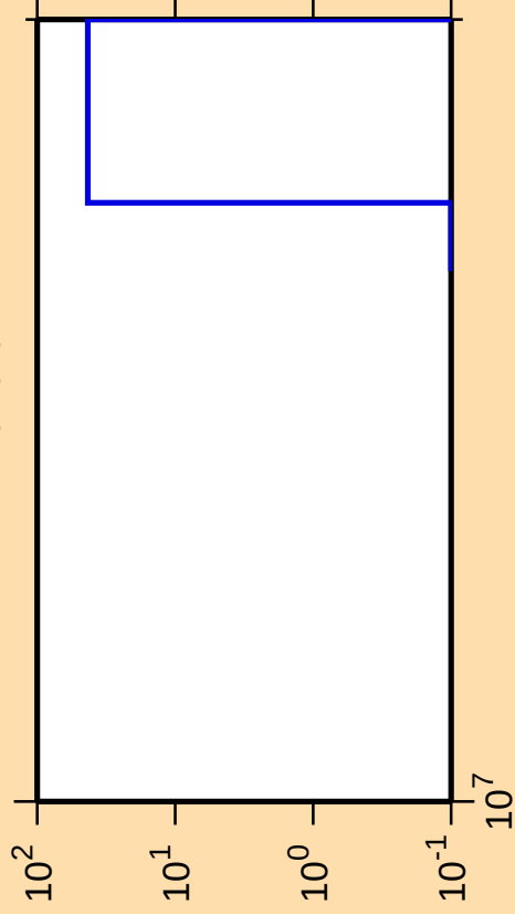
\Delta\sigma/\sigma vs. E for ^{131}\text{Ba}(n,\text{pt})
