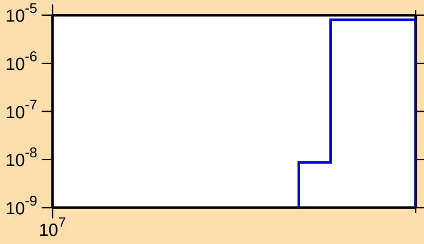
\sigma vs. E for ^{131}\text{Ba}(n,2np)
