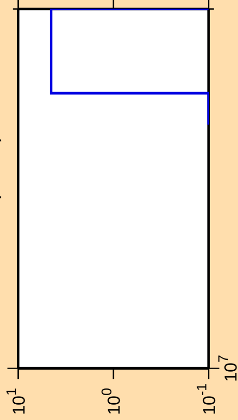
\Delta\sigma/\sigma vs. E for ^{131}\text{Ba} (mt 34)
