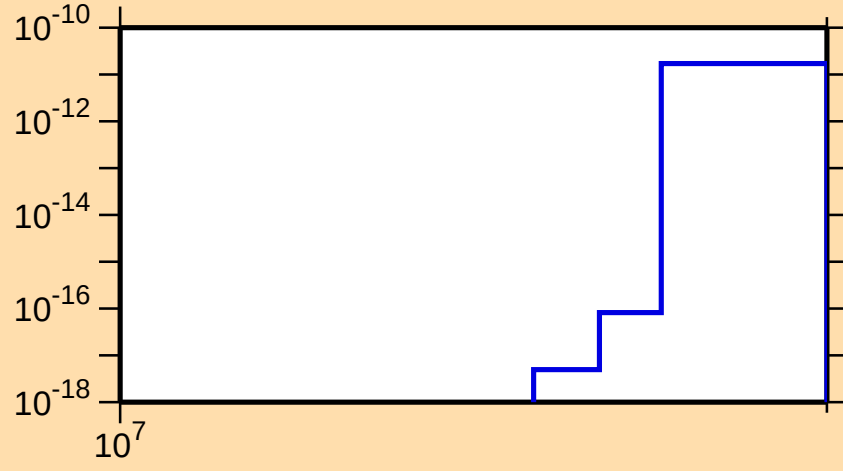
\sigma vs. E for ^{131}\text{Ba}(n,\text{nt})
