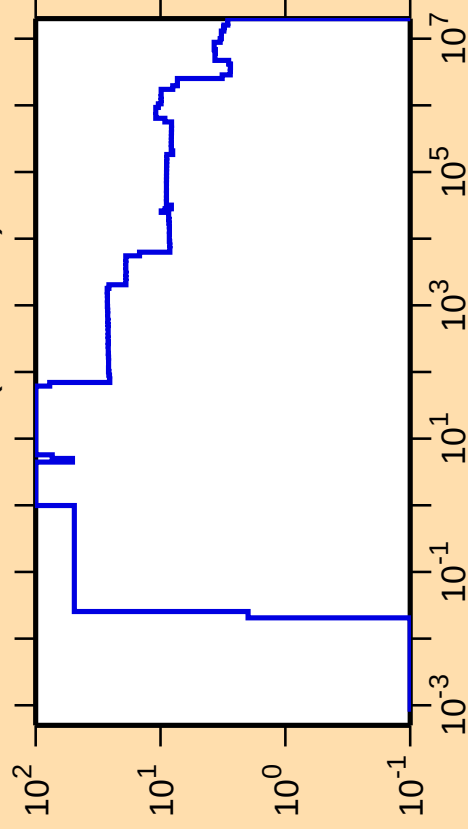
\Delta\sigma/\sigma vs. E for ^{131}\text{Ba}(n,\text{nonel.})
