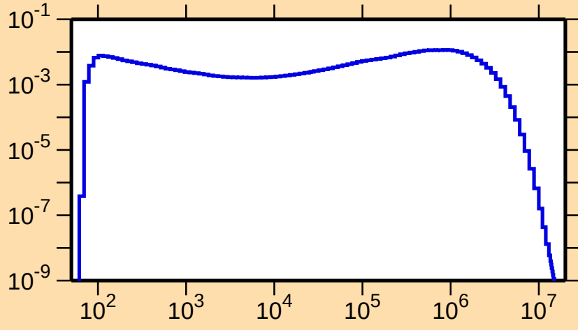
\sigma vs. E for ^{131}\text{Ba}(n,n_1)
