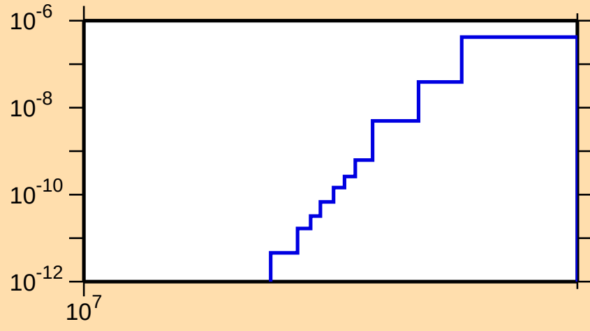
\sigma vs. E for ^{131}\text{Ba}(n,\text{He}3)
