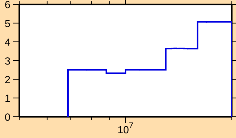
\Delta\sigma/\sigma vs. E for ^{131}\text{Ba}(n,\text{el.})
