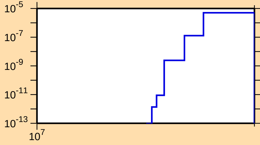
\sigma vs. E for ^{131}\text{Ba}(n,\text{nd})
