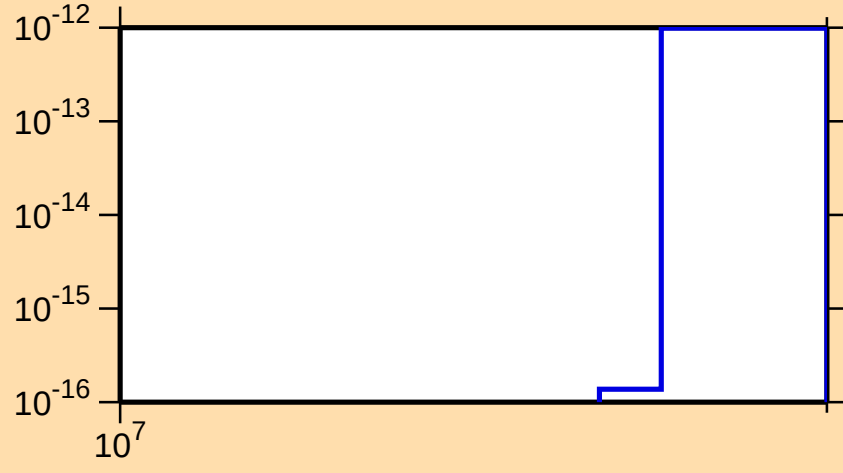
\sigma vs. E for ^{131}\text{Ba} (mt 34)
