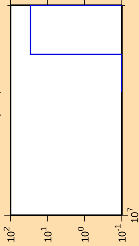
\Delta\sigma/\sigma vs. E for ^{131}\text{Ba}(n,\text{nt})
