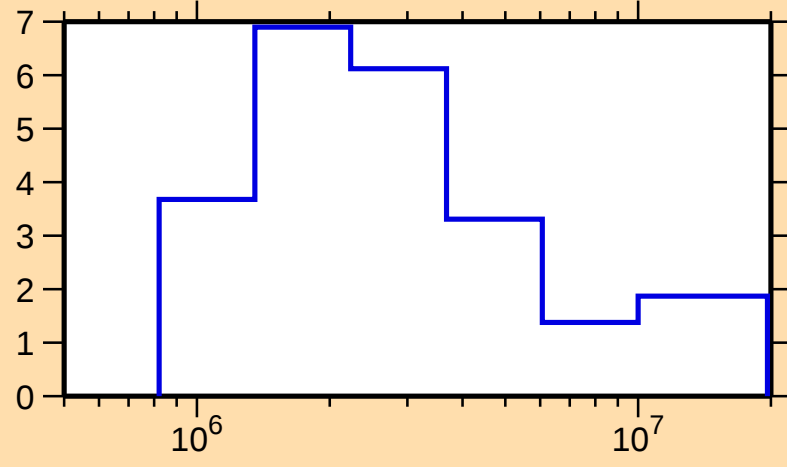
\Delta\sigma/\sigma vs. E for ^{131}\text{Ba}(n,\text{tot.})
