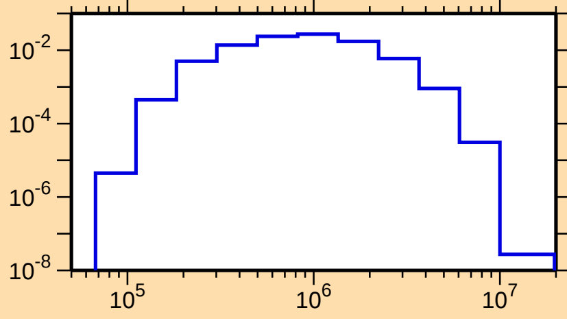
\sigma vs. E for ^{131}\text{Ba}(n,n_3)
