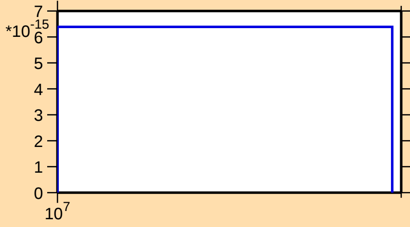
\sigma vs. E for ^{131}\text{Ba} (mt 34)
