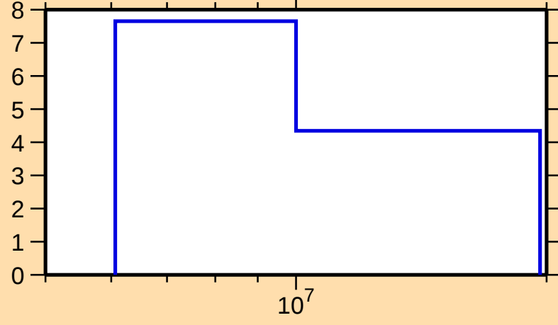
\Delta\sigma/\sigma vs. E for ^{131}\text{Ba}(n,2n)
