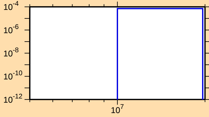
\sigma vs. E for ^{131}\text{Ba}(n,t)
