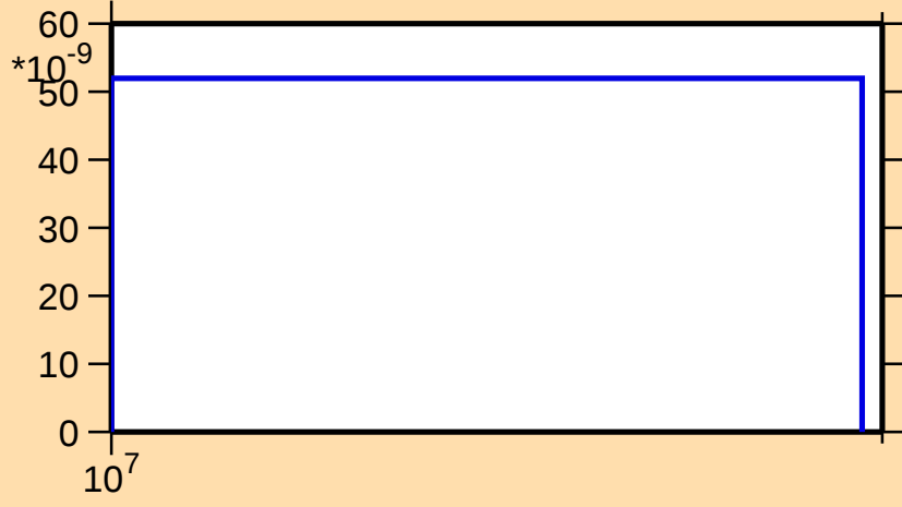
\sigma vs. E for ^{131}\text{Ba}(n,\text{nd})
