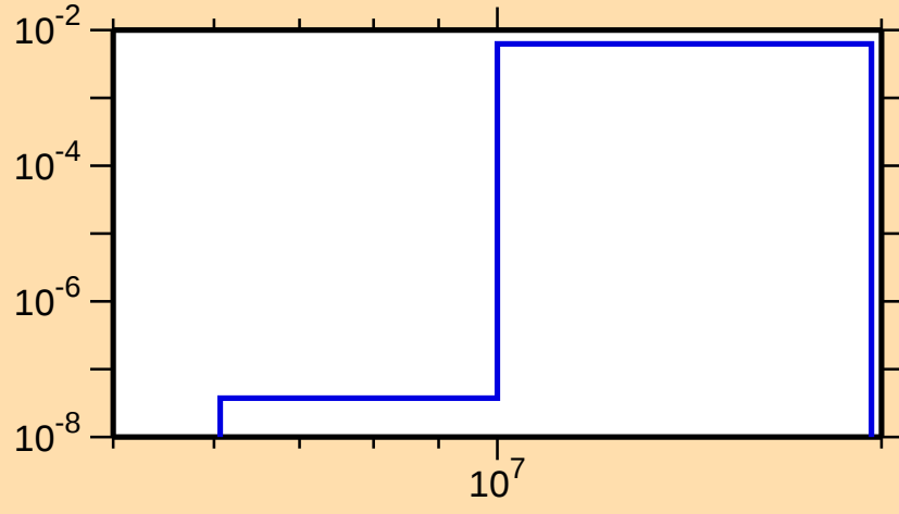
\sigma vs. E for ^{131}\text{Ba}(n,np)
