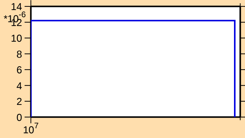
\sigma vs. E for ^{131}\text{Ba}(n,3n)
