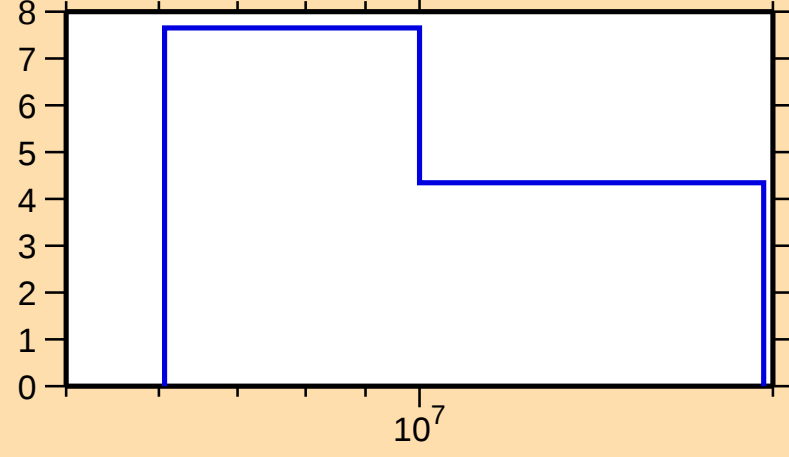
\Delta\sigma/\sigma vs. E for ^{131}\text{Ba}(n,2n)
