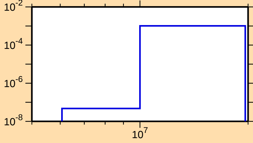
\sigma vs. E for ^{131}\text{Ba}(n,n\alpha)
