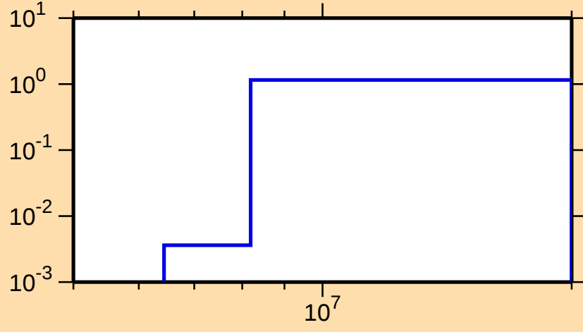
\sigma vs. E for ^{131}\text{Ba}(n,2n)
