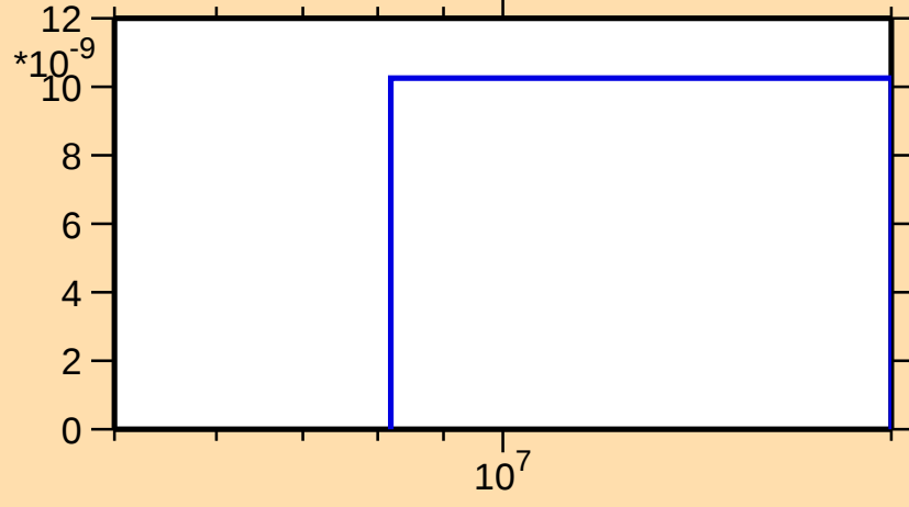
\sigma vs. E for ^{131}\text{Ba}(n,2n\alpha)
