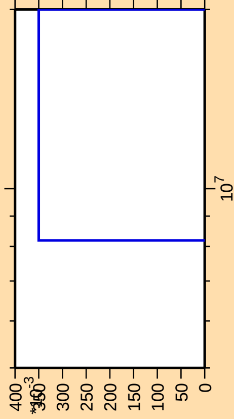
\Delta\sigma/\sigma vs. E for ^{131}\text{Ba}(n,\text{pt})
