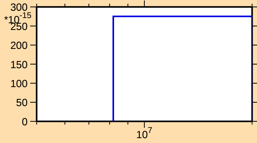
\sigma vs. E for ^{131}\text{Ba}(n,\text{pt})
