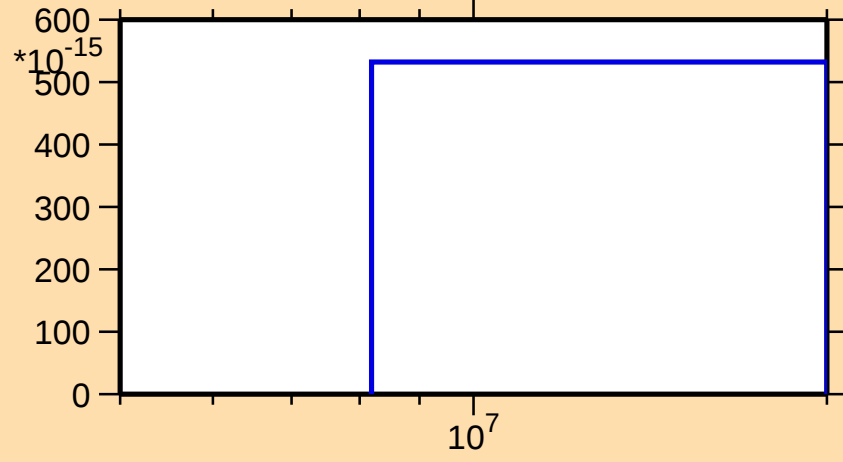
\sigma vs. E for ^{131}\text{Ba}(n,\text{pd})
