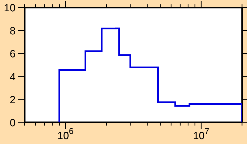
\Delta\sigma/\sigma vs. E for ^{131}\text{Ba}(n,\text{tot.})
