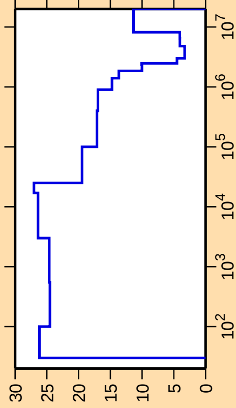
\Delta\sigma/\sigma vs. E for ^{131}\text{Ba}(n,\text{inel.})
