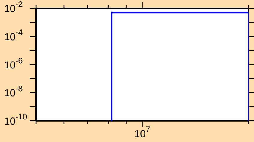
\sigma vs. E for ^{131}\text{Ba}(n,np)
