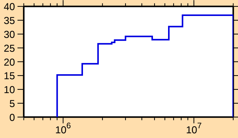
\Delta\sigma/\sigma vs. E for ^{131}\text{Ba}(n,n_1)
