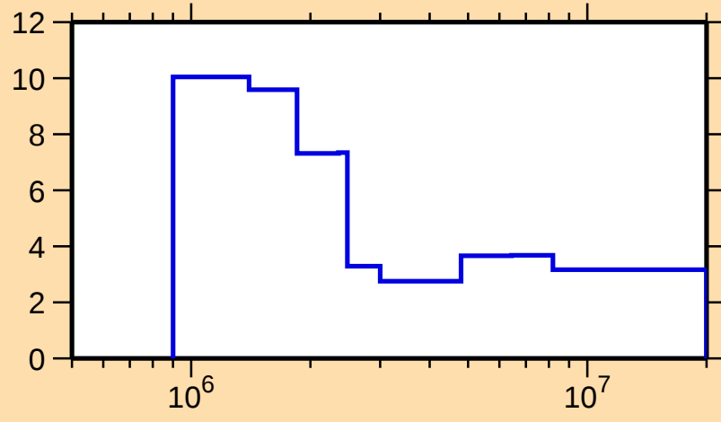
\Delta\sigma/\sigma vs. E for ^{131}\text{Ba}(n,\text{nonel.})
