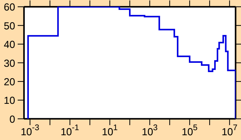
\Delta\sigma/\sigma vs. E for ^{131}\text{Ba}(n,p)
