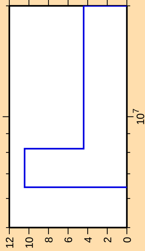
\Delta\sigma/\sigma vs. E for ^{131}\text{Ba}(n,2n)
