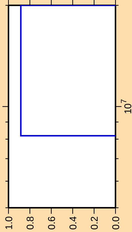
\Delta\sigma/\sigma vs. E for ^{131}\text{Ba}(n,\text{pd})
