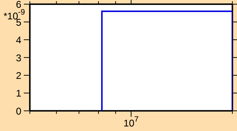
\sigma vs. E for ^{131}\text{Ba}(n,\text{He}3)
