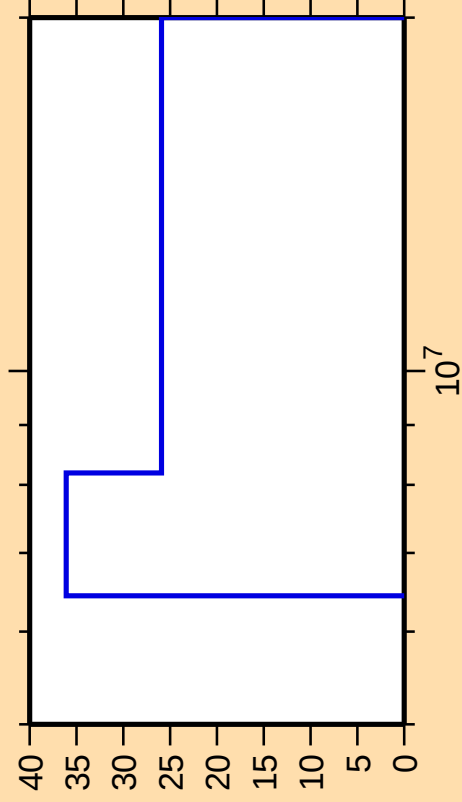
\Delta\sigma/\sigma vs. E for ^{131}\text{Ba}(n,p)
