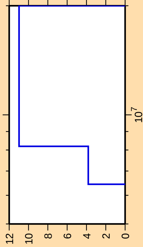
\Delta\sigma/\sigma vs. E for ^{131}\text{Ba}(n,n\text{cont.})
