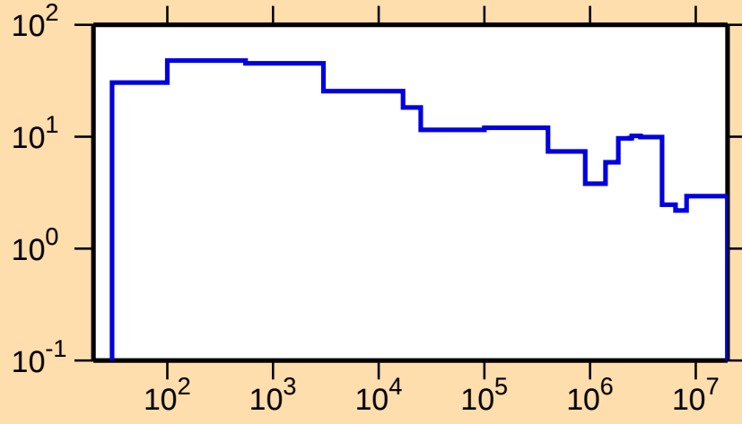
\Delta\sigma/\sigma vs. E for ^{131}\text{Ba}(n,\text{el.})
