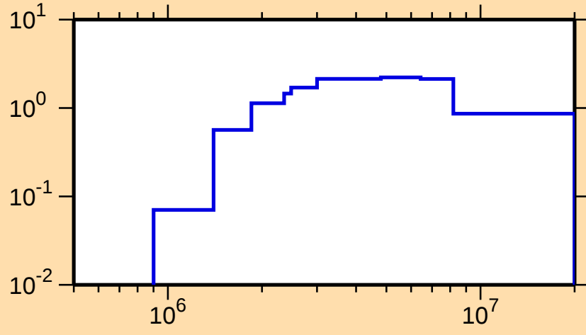
\sigma vs. E for ^{131}\text{Ba}(n,n\text{cont.})
