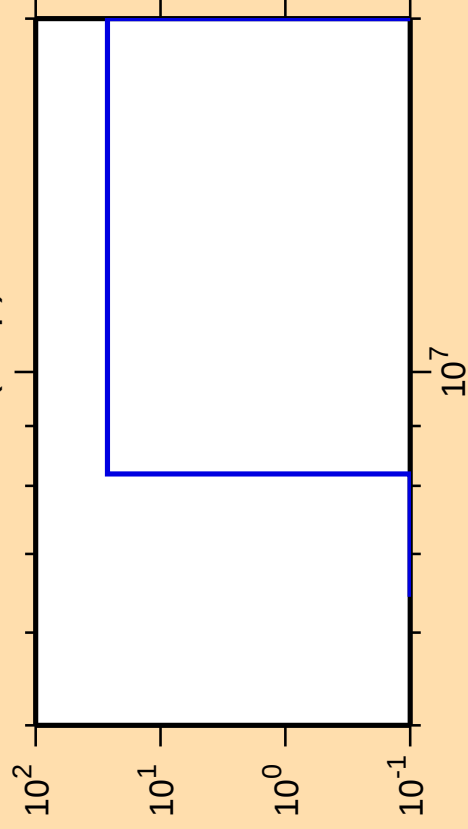
\Delta\sigma/\sigma vs. E for ^{131}\text{Ba}(n,np)
