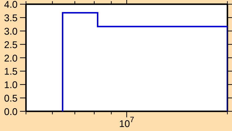
\Delta\sigma/\sigma vs. E for ^{131}\text{Ba}(n,\text{nonel.})
