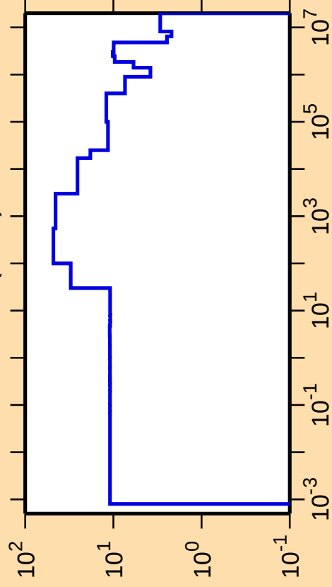
\Delta\sigma/\sigma vs. E for ^{131}\text{Ba}(n,\text{el.})
