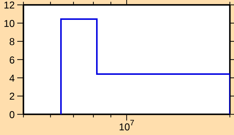
\Delta\sigma/\sigma vs. E for ^{131}\text{Ba}(n,2n)
