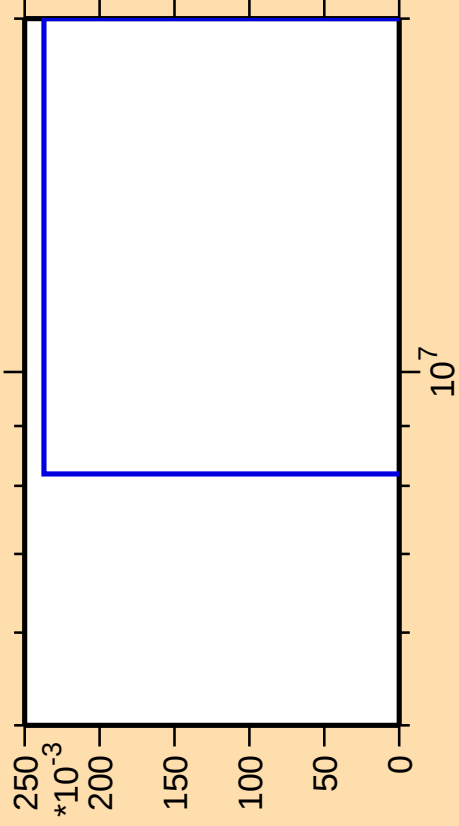
\Delta\sigma/\sigma vs. E for ^{131}\text{Ba}(n,nt)
