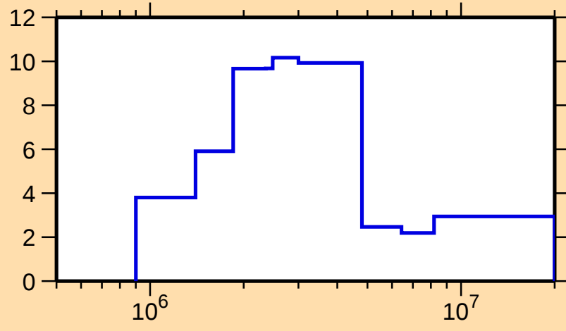
\Delta\sigma/\sigma vs. E for ^{131}\text{Ba}(n,\text{el.})
