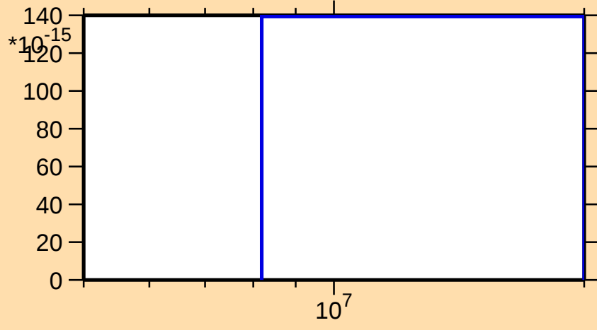
\sigma vs. E for ^{131}\text{Ba}(n,nt)
