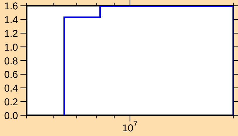
\Delta\sigma/\sigma vs. E for ^{131}\text{Ba}(n,\text{tot.})
