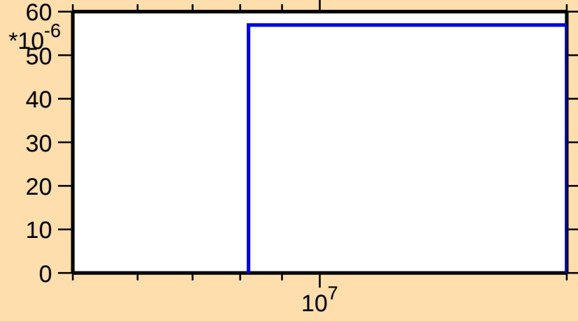
\sigma vs. E for ^{131}\text{Ba}(n,t)
