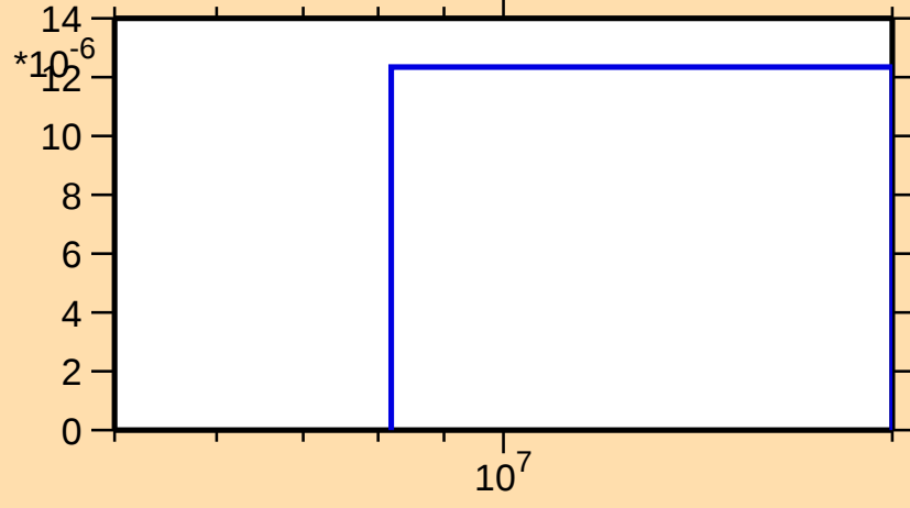
\sigma vs. E for ^{131}\text{Ba}(n,3n)
