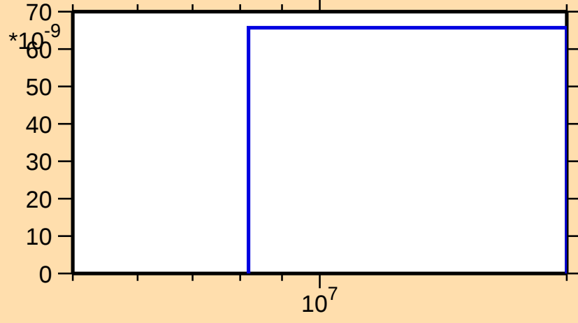
\sigma vs. E for ^{131}\text{Ba}(n,2np)
