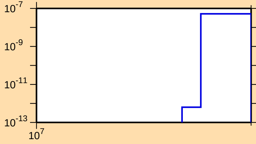
\sigma vs. E for ^{135}\text{Ba}(n,2np)
