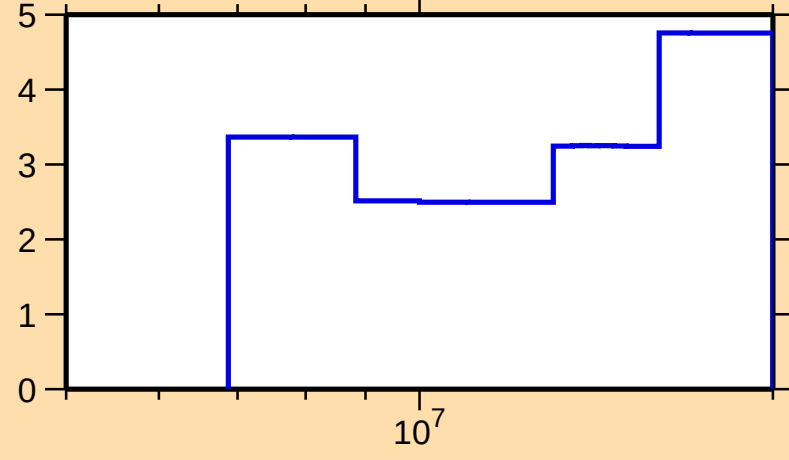
\Delta\sigma/\sigma vs. E for ^{135}\text{Ba}(n,\text{el.})
