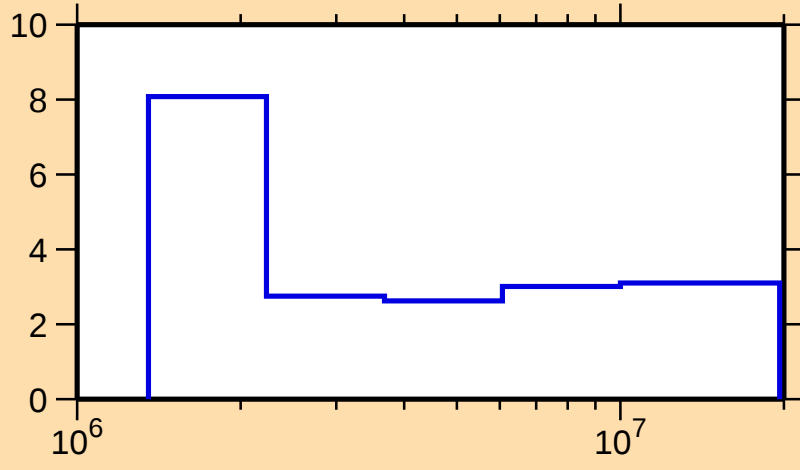
\Delta\sigma/\sigma vs. E for ^{135}\text{Ba}(n,\text{nonel.})
