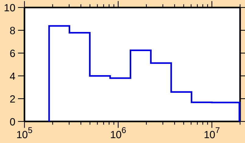
\Delta\sigma/\sigma vs. E for ^{135}\text{Ba}(n,\text{tot.})
