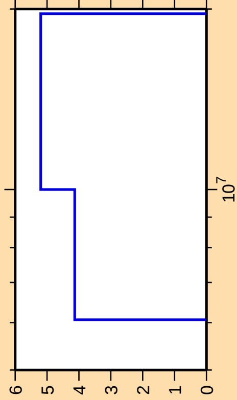
\Delta\sigma/\sigma vs. E for ^{135}\text{Ba}(n,n\text{cont.})
