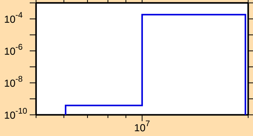
\sigma vs. E for ^{135}\text{Ba}(n,n\alpha)
