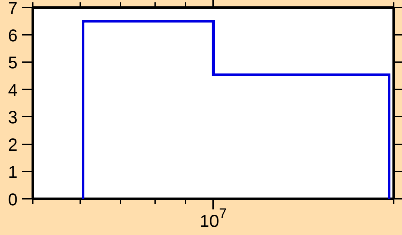
\Delta\sigma/\sigma vs. E for ^{135}\text{Ba}(n,2n)
