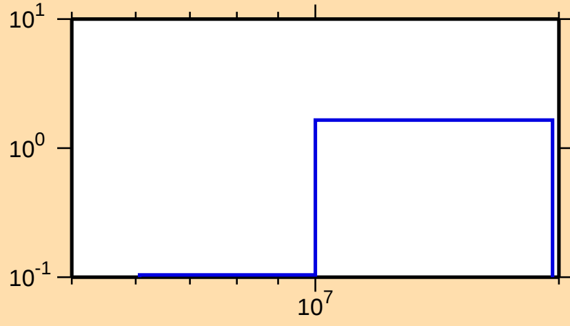
\sigma vs. E for ^{135}\text{Ba}(n,2n)
