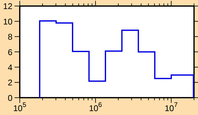
\Delta\sigma/\sigma vs. E for ^{135}\text{Ba}(n,\text{el.})
