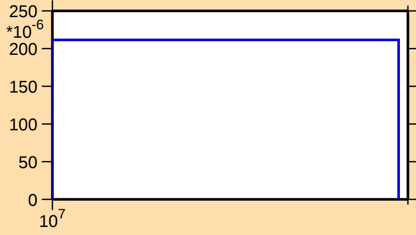
\sigma vs. E for ^{135}\text{Ba}(n,3n)
