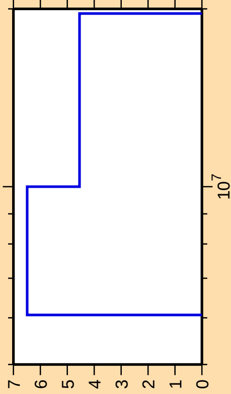
\Delta\sigma/\sigma vs. E for ^{135}\text{Ba}(n,2n)
