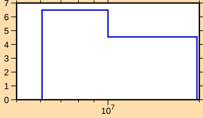
\Delta\sigma/\sigma vs. E for ^{135}\text{Ba}(n,2n)
