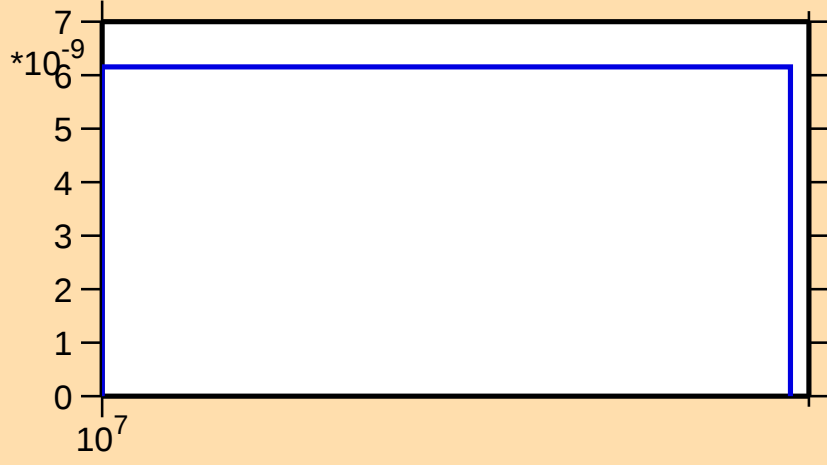
\sigma vs. E for ^{135}\text{Ba}(n,\text{nd})
