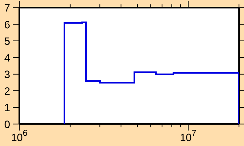
\Delta\sigma/\sigma vs. E for ^{135}\text{Ba}(n,\text{nonel.})
