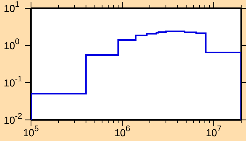
\sigma vs. E for ^{135}\text{Ba}(n,\text{inel.})
