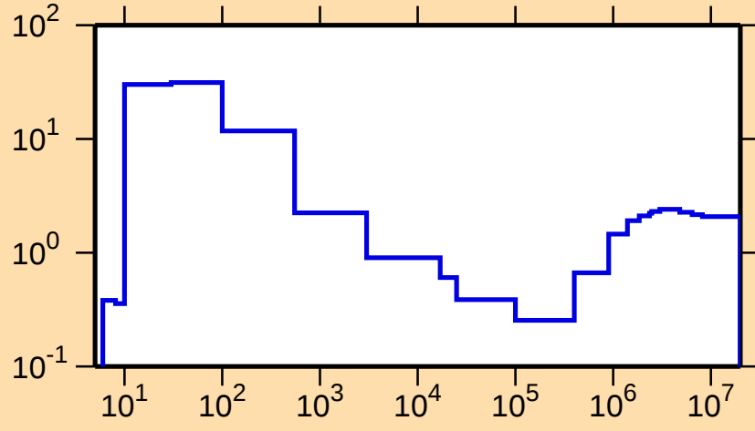
\sigma vs. E for ^{135}\text{Ba}(n,\text{nonel.})
