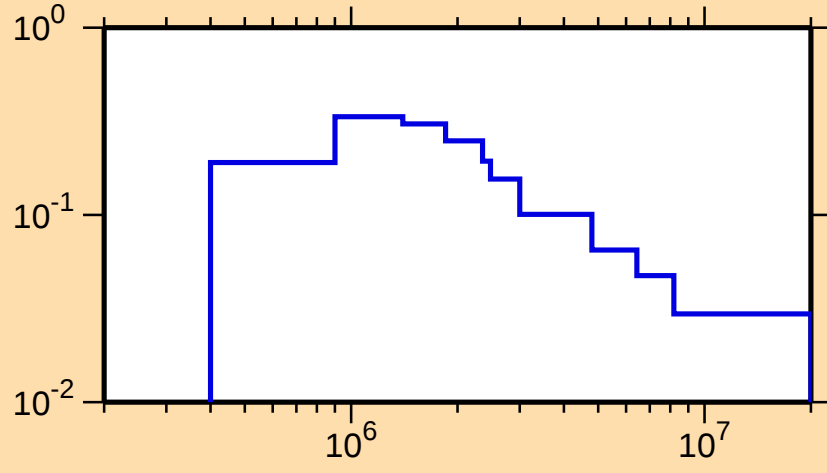
\sigma vs. E for ^{135}\text{Ba}(n,n_3)
