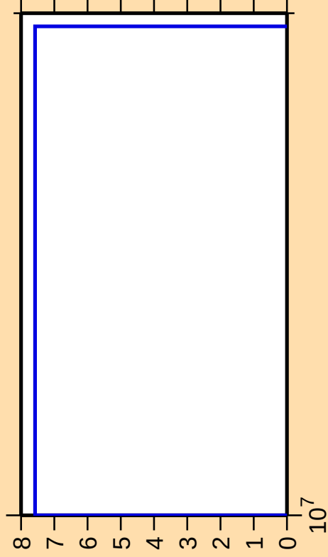
\Delta\sigma/\sigma vs. E for ^{137}\text{Ba}(n,\text{nt})
