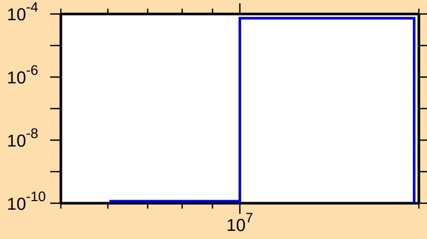
\sigma vs. E for ^{137}\text{Ba}(n,n\alpha)
