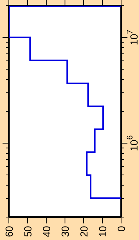
\Delta\sigma/\sigma vs. E for ^{137}\text{Ba}(n,n_4)
