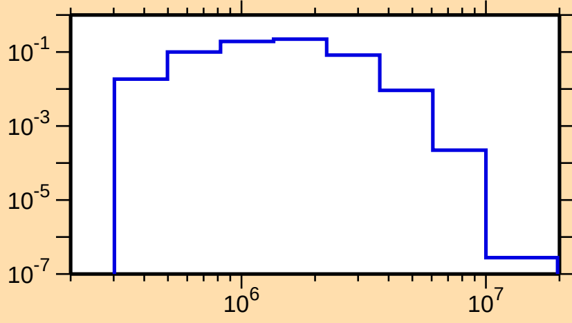
\sigma vs. E for ^{137}\text{Ba}(n,n_4)
