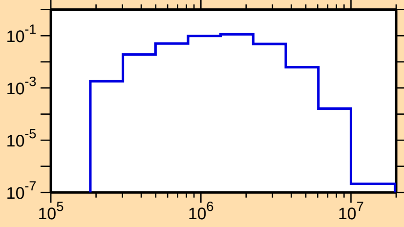
\sigma vs. E for ^{137}\text{Ba}(n,n_3)
