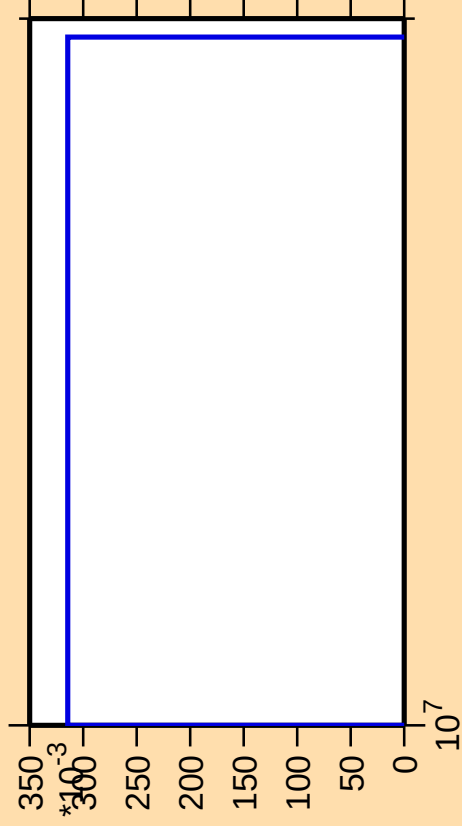
\Delta\sigma/\sigma vs. E for ^{137}\text{Ba}(n,p\alpha)
