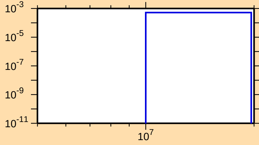
\sigma vs. E for ^{137}\text{Ba}(n,np)
