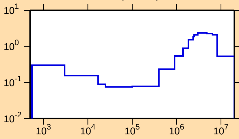
\sigma vs. E for ^{137}\text{Ba}(n,\text{inel.})
