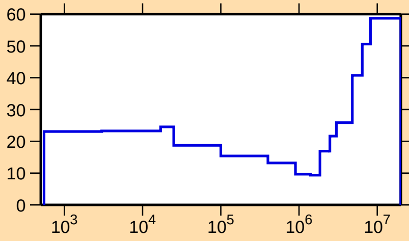
\Delta\sigma/\sigma vs. E for ^{137}\text{Ba}(n,n_1)
