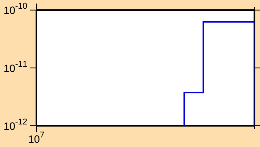
\sigma vs. E for ^{143}\text{Ba}(n,3n\alpha)
