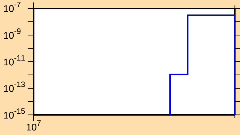
\sigma vs. E for ^{143}\text{Ba}(n,2np)
