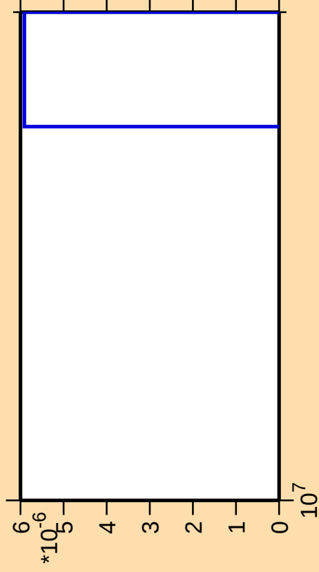
\Delta\sigma/\sigma vs. E for ^{143}\text{Ba} (mt 11)
