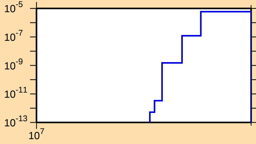
\sigma vs. E for ^{143}\text{Ba}(n,nt)
