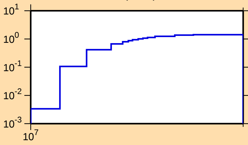
\sigma vs. E for ^{143}\text{Ba}(n,3n)
