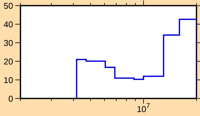
\Delta\sigma/\sigma vs. E for ^{143}\text{Ba}(n,2n)
