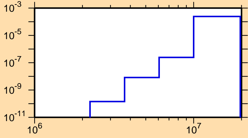
\sigma vs. E for ^{143}\text{Ba}(n,\alpha)
