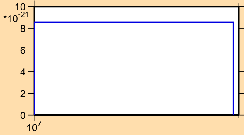
\sigma vs. E for ^{143}\text{Ba} (mt 11)
