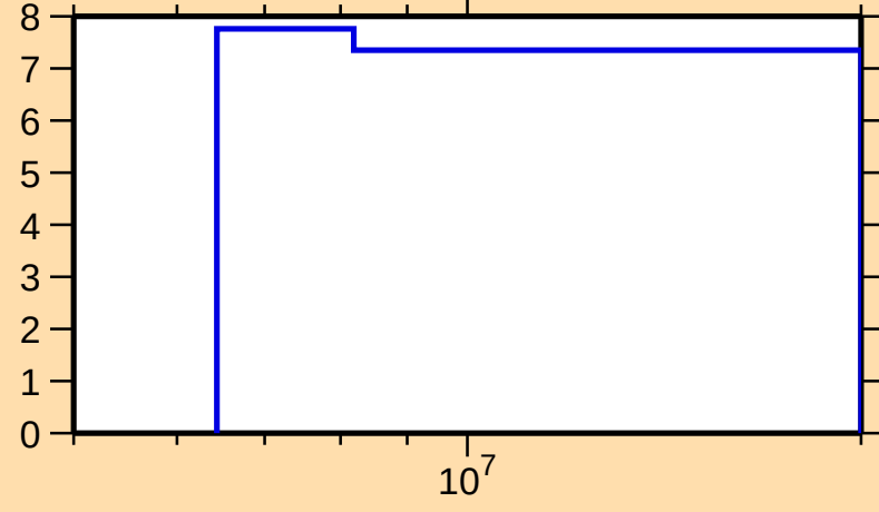
\Delta\sigma/\sigma vs. E for ^{143}\text{Ba}(n,\text{nonel.})
