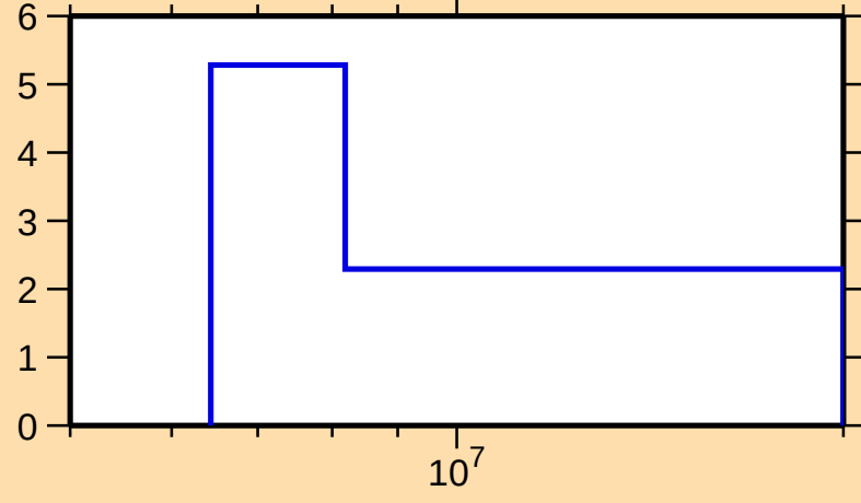
\Delta\sigma/\sigma vs. E for ^{143}\text{Ba}(n,\text{tot.})
