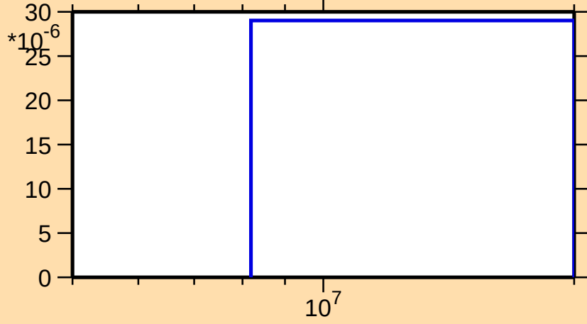
\sigma vs. E for ^{143}\text{Ba}(n,t)
