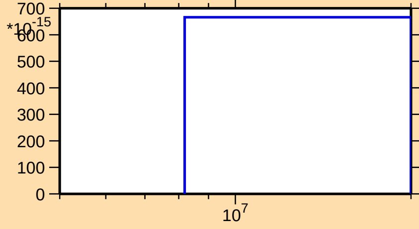
\sigma vs. E for ^{143}\text{Ba}(n,3n\alpha)
