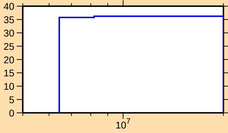
\Delta\sigma/\sigma vs. E for ^{143}\text{Ba}(n,n\text{cont.})
