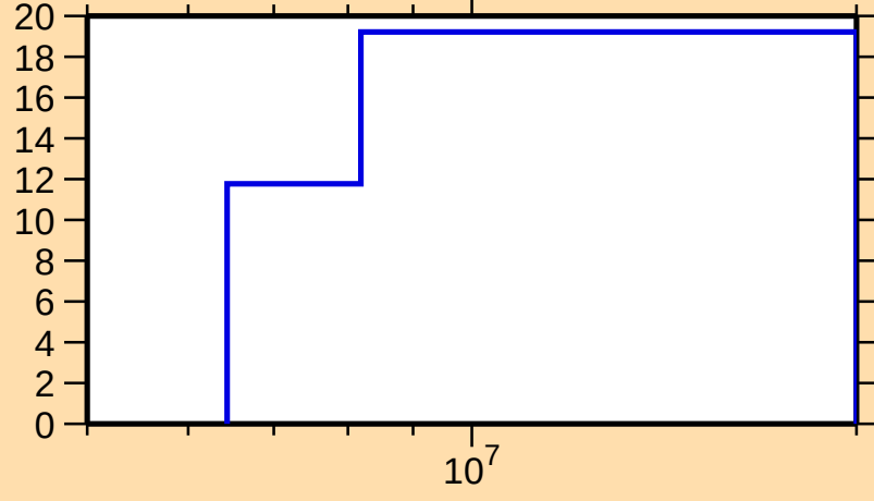
\Delta\sigma/\sigma vs. E for ^{143}\text{Ba}(n,2n)
