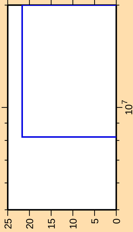
\Delta\sigma/\sigma vs. E for ^{143}\text{Ba}(n,3n)
