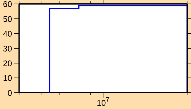
\Delta\sigma/\sigma vs. E for ^{143}\text{Ba}(n,\gamma)
