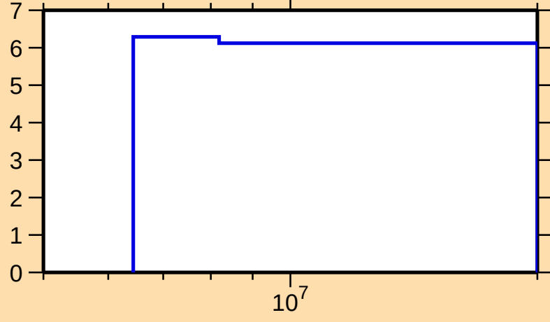
\Delta\sigma/\sigma vs. E for ^{143}\text{Ba}(n,\text{el.})
