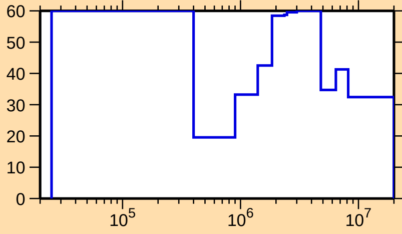
\Delta\sigma/\sigma vs. E for ^{143}\text{Ba}(n,n_1)
