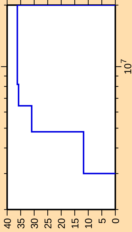
\Delta\sigma/\sigma vs. E for ^{143}\text{Ba}(n,n\text{cont.})
