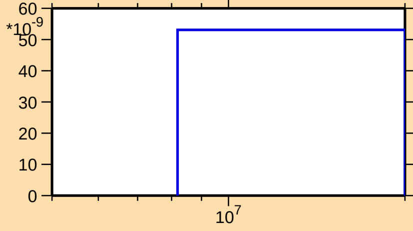
\sigma vs. E for ^{143}\text{Ba}(n,nt)
