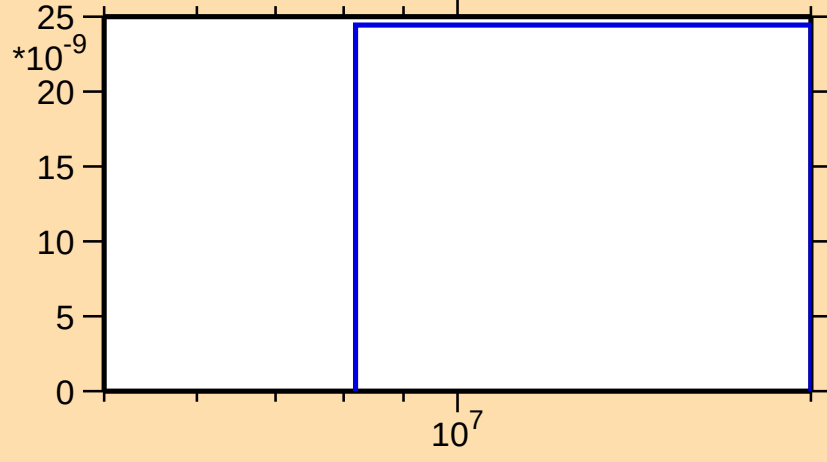
\sigma vs. E for ^{143}\text{Ba}(n,\text{nd})
