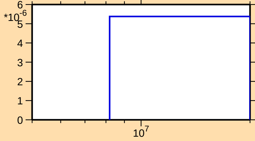
\sigma vs. E for ^{143}\text{Ba}(n,np)
