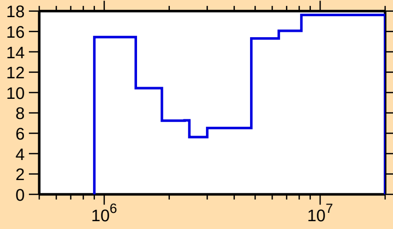
\Delta\sigma/\sigma vs. E for ^{143}\text{Ba}(n,\text{inel.})
