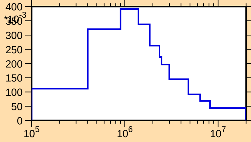
\sigma vs. E for ^{143}\text{Ba}(n,n_2)
