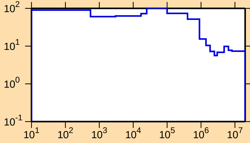
\Delta\sigma/\sigma vs. E for ^{143}\text{Ba}(n,\text{nonel.})
