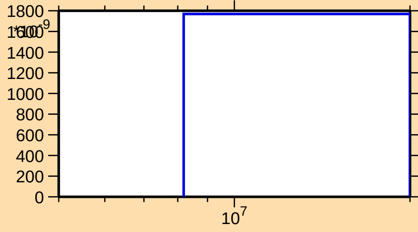
\sigma vs. E for ^{264}\alpha )
