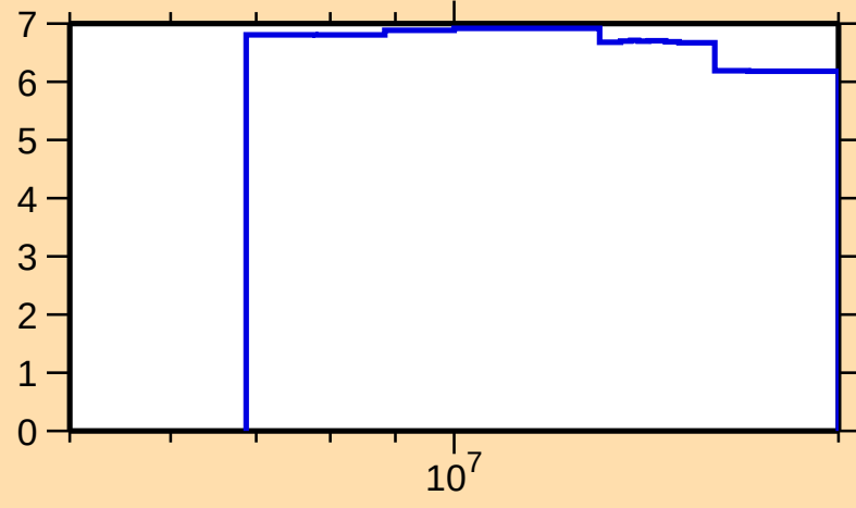
\Delta\sigma/\sigma vs. E for ^{267}
