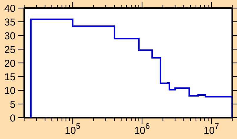
\Delta\sigma/\sigma vs. E for ^{268}\text{Po}
