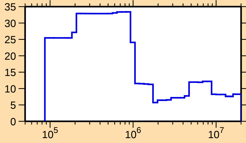
\Delta\sigma/\sigma vs. E for ^{271}\text{I}
