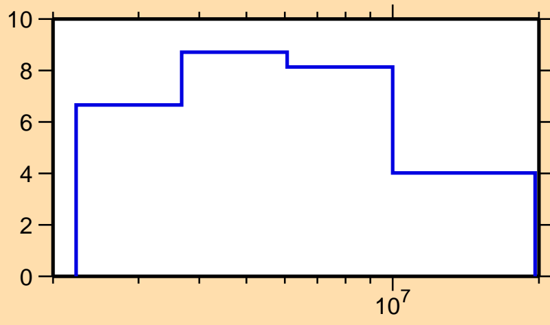
\Delta\sigma/\sigma vs. E for ^{214}\text{Bi}(n,el.)
