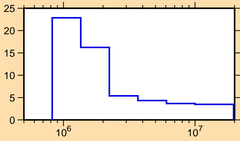
\Delta\sigma/\sigma vs. E for ^{214}\text{Bi}(n,n\text{onel.})
