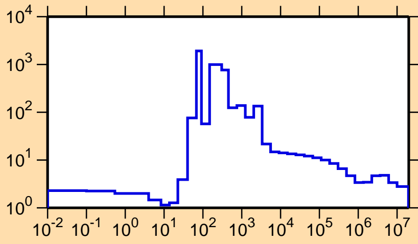
\sigma vs. E for ^{214}\text{Bi}(n,\text{el.})
