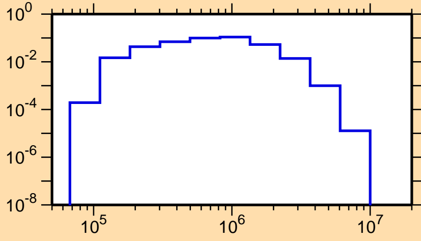
\sigma vs. E for ^{214}\text{Bi}(n,n_3)
