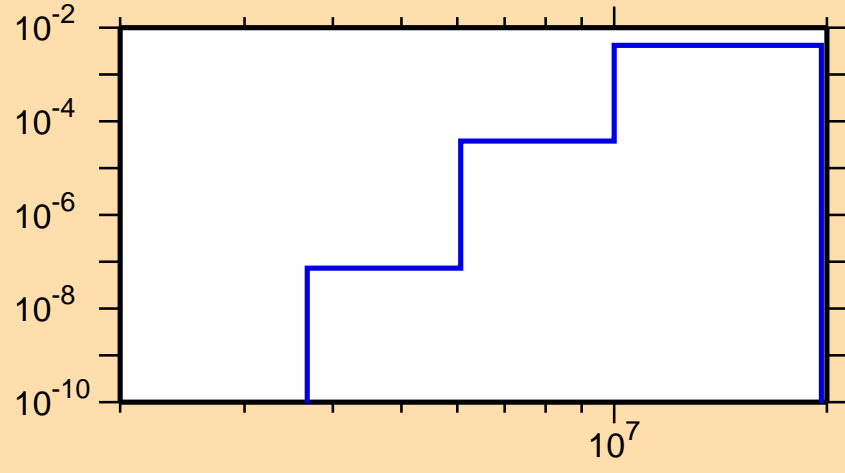
\sigma vs. E for ^{214}\text{Bi}(n,p)
