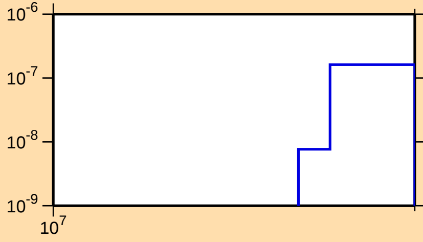
\sigma vs. E for ^{235}\text{Bk}(n,nt)
