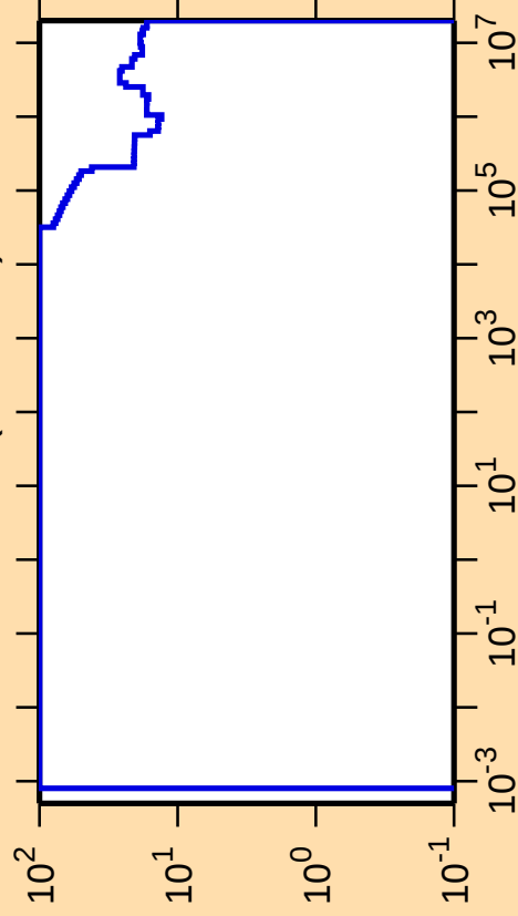
\Delta\sigma/\sigma vs. E for ^{235}\text{Bk}(n,\text{nonel.})
