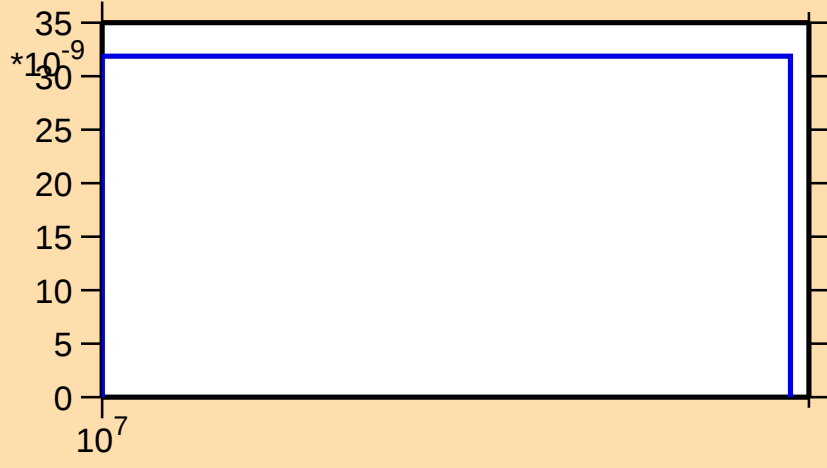
\sigma vs. E for ^{235}\text{Bk}(n,\text{nd})
