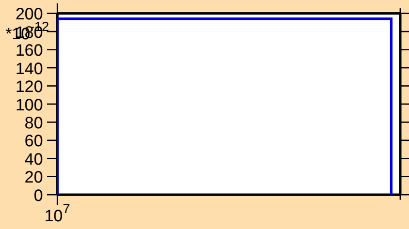
\sigma vs. E for ^{235}\text{Bk}(n,3n)
