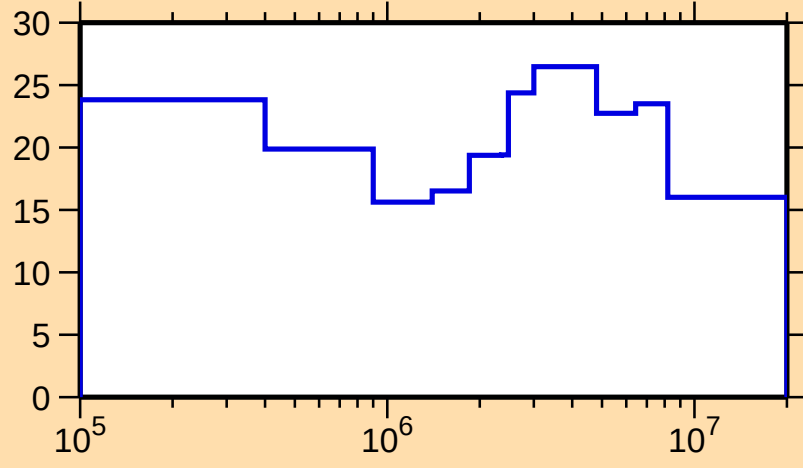
\Delta\sigma/\sigma vs. E for ^{235}\text{Bk}(n,f)
