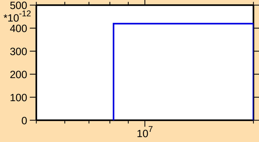
\sigma vs. E for ^{235}\text{Bk}(n,p\alpha)
