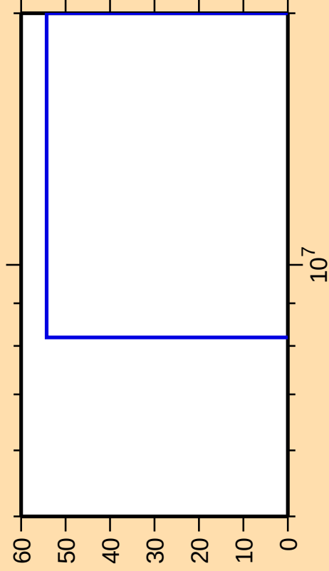
\Delta\sigma/\sigma vs. E for ^{235}\text{Bk}(n,n_1)
