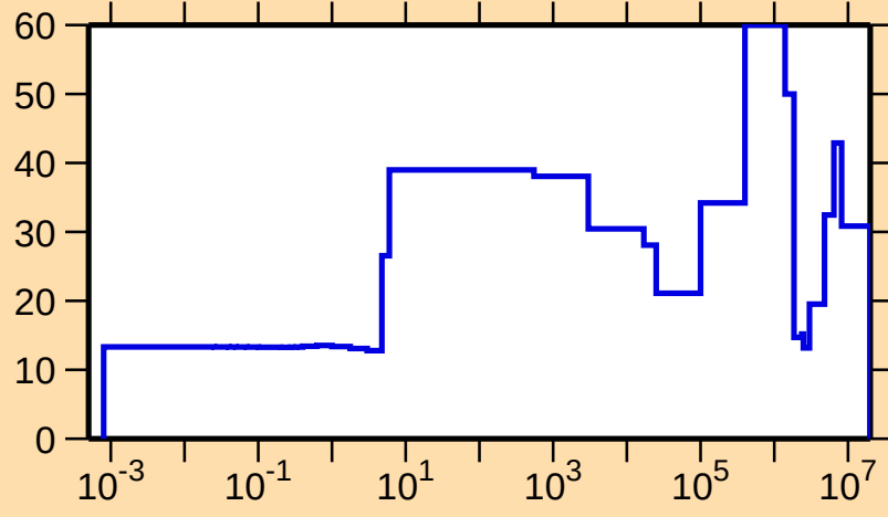
\Delta\sigma/\sigma vs. E for ^{235}\text{Bk}(n,\text{el.})
