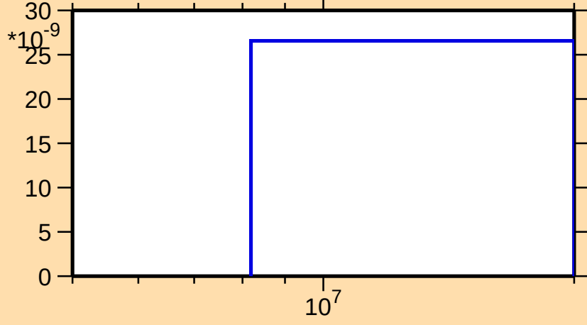
\sigma vs. E for ^{235}\text{Bk}(n,\text{nd})
