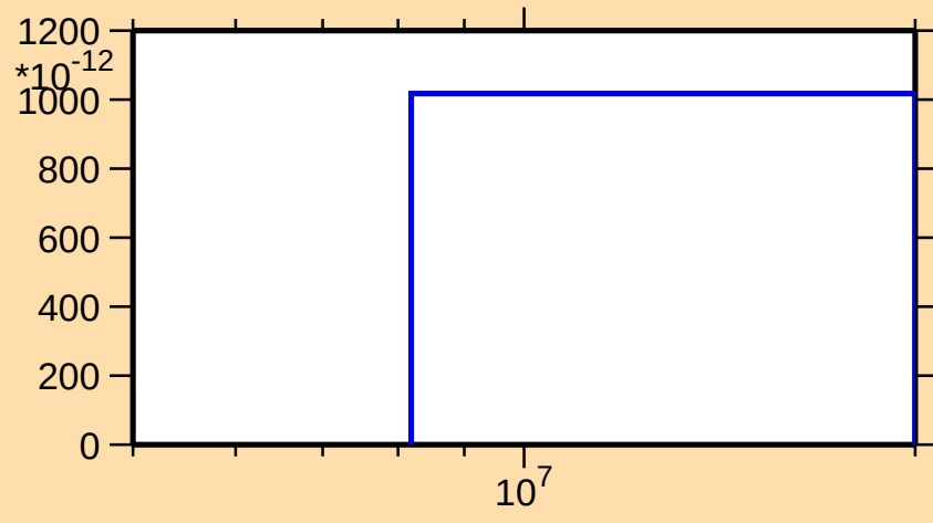
\sigma vs. E for ^{235}\text{Bk}(n,\text{He}3)
