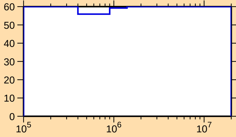
\Delta\sigma/\sigma vs. E for ^{235}\text{Bk}(n,\text{inel.})
