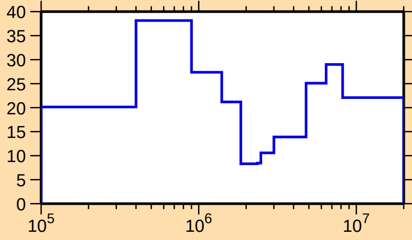
\Delta\sigma/\sigma vs. E for ^{235}\text{Bk}(n,\text{tot.})
