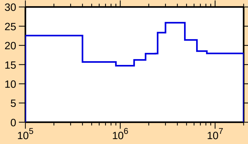
\Delta\sigma/\sigma vs. E for ^{235}\text{Bk}(n,\text{nonel.})
