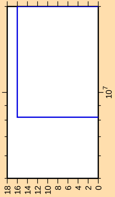
\Delta\sigma/\sigma vs. E for ^{235}\text{Bk}(n,f)
