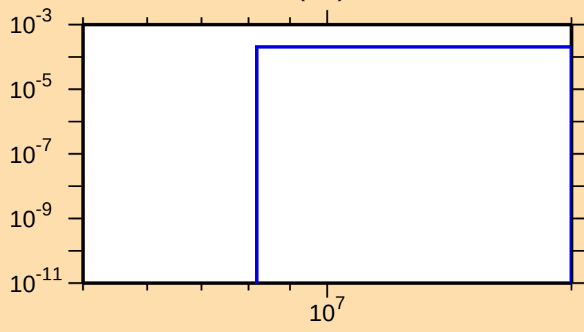
\sigma vs. E for ^{235}\text{Bk}(n,t)
