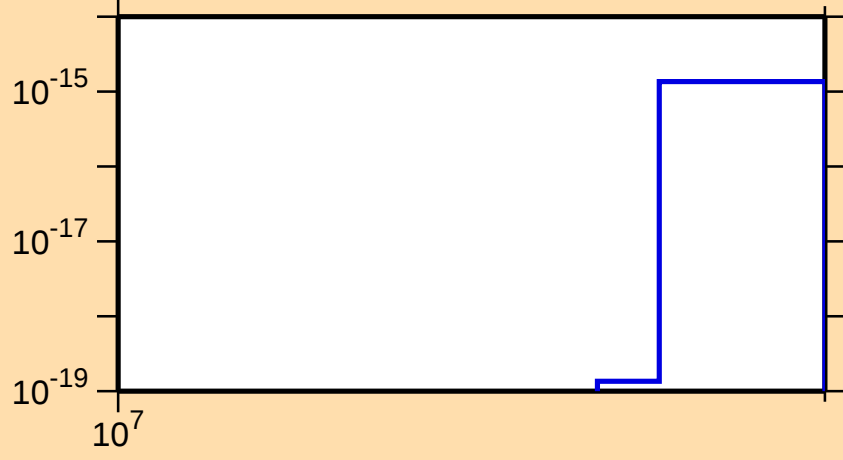
\sigma vs. E for ^{236}\text{Bk}(n,3n\alpha)
