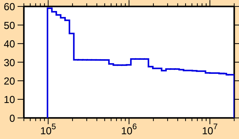
\Delta\sigma/\sigma vs. E for ^{236}\text{Bk}(n,f)
