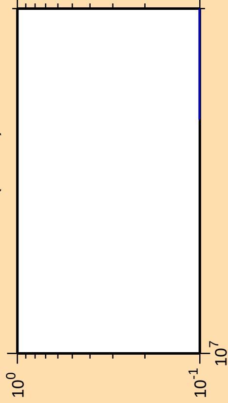
\Delta\sigma/\sigma vs. E for ^{236}\text{Bk}(n,3n\alpha)
