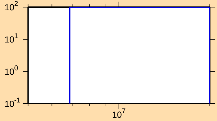
\Delta\sigma/\sigma vs. E for ^{236}\text{Bk}(n,2n)
