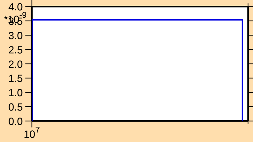
\sigma vs. E for ^{236}\text{Bk}(n,3n)
