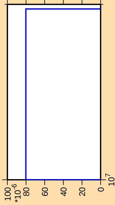
\Delta\sigma/\sigma vs. E for ^{236}\text{Bk}(n,3n\alpha)
