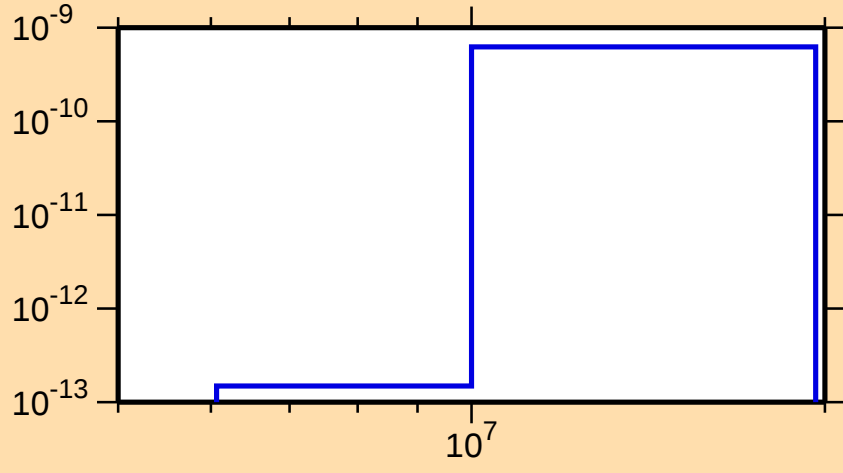
\sigma vs. E for ^{236}\text{Bk}(n,p\alpha)
