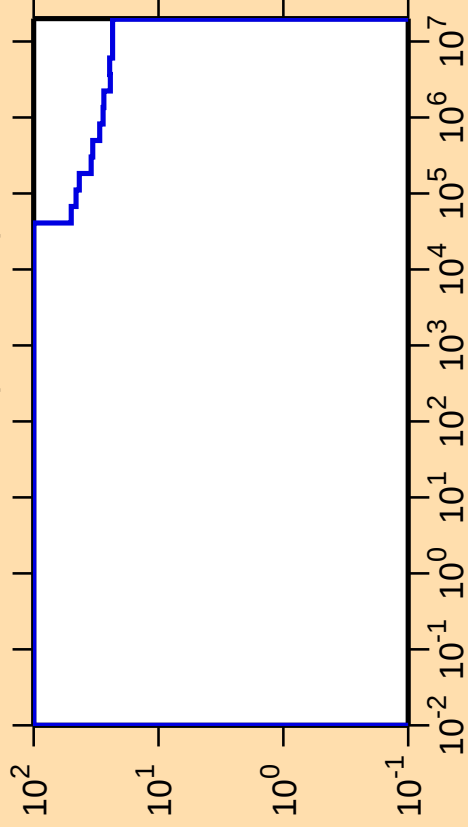
\Delta\sigma/\sigma vs. E for ^{236}\text{Bk}(n,\text{nonel.})
