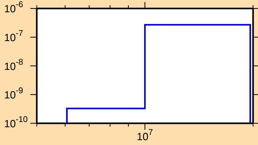
\sigma vs. E for ^{236}\text{Bk}(n,t)
