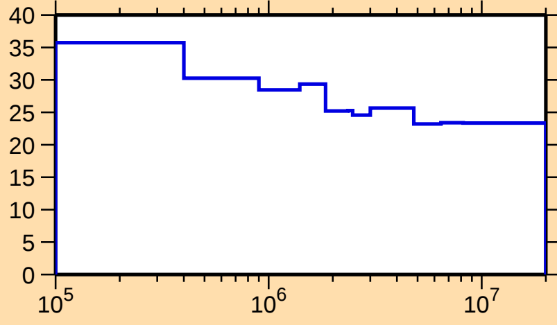
\Delta\sigma/\sigma vs. E for ^{236}\text{Bk}(n,\text{nonel.})
