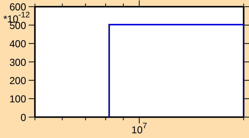
\sigma vs. E for ^{236}\text{Bk}(n,p\alpha)
