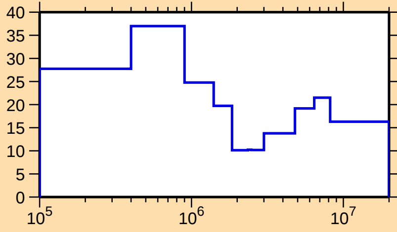
\Delta\sigma/\sigma vs. E for ^{236}\text{Bk}(n,\text{tot.})
