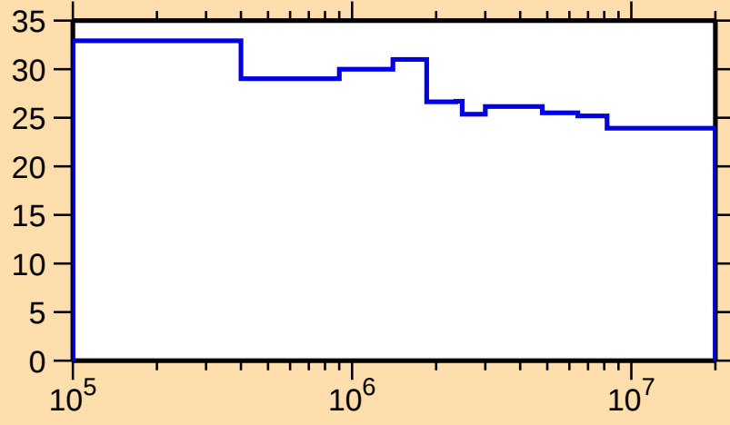
\Delta\sigma/\sigma vs. E for ^{236}\text{Bk}(n,f)
