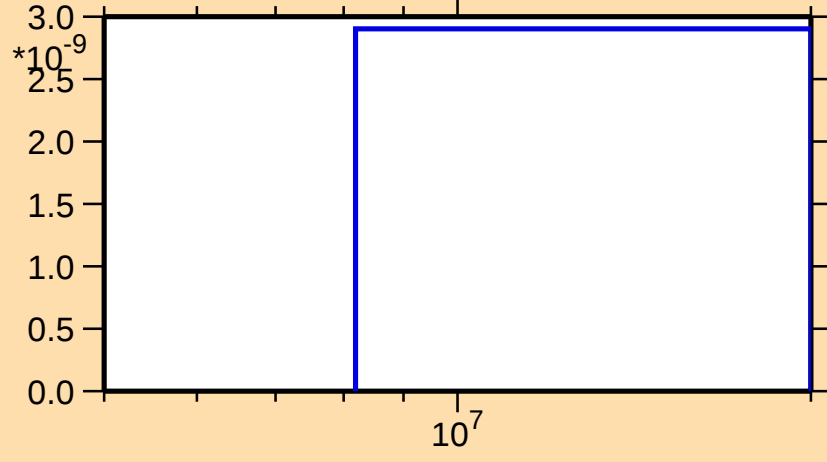
\sigma vs. E for ^{236}\text{Bk}(n,\text{He}3)
