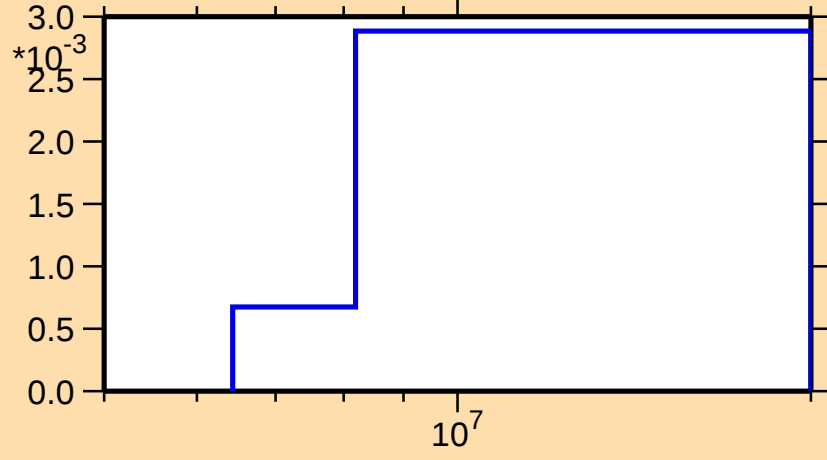
\sigma vs. E for ^{236}\text{Bk}(n,2n)
