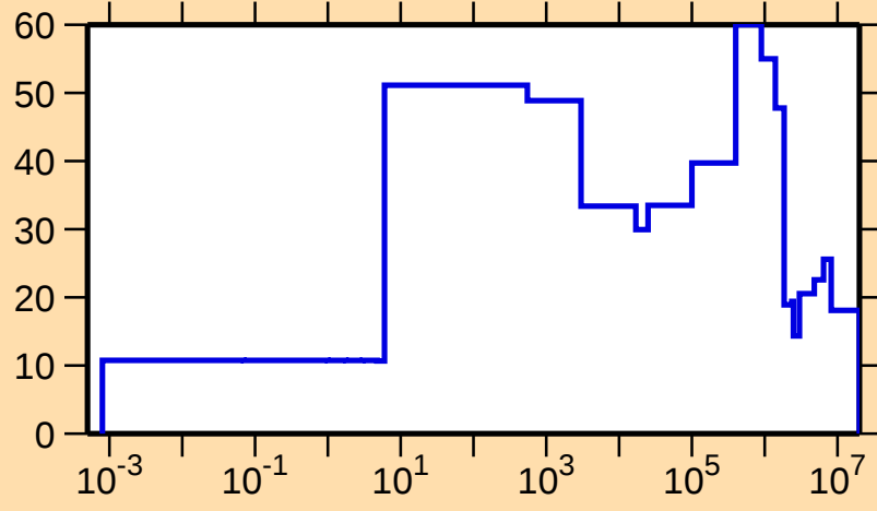
\Delta\sigma/\sigma vs. E for ^{236}\text{Bk}(n,\text{el.})
