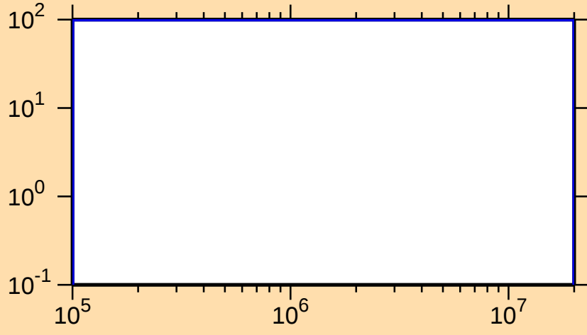
\Delta\sigma/\sigma vs. E for ^{236}\text{Bk}(n,\text{ncont.})
