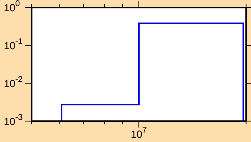
\sigma vs. E for ^{239}\text{Bk}(n,2n)
