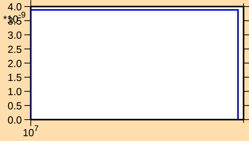
\sigma vs. E for ^{239}\text{Bk}(n,\text{nd})
