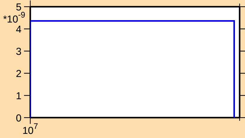
\sigma vs. E for ^{239}\text{Bk}(n,2np)
