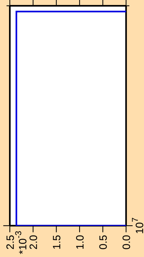
\Delta\sigma/\sigma vs. E for ^{239}\text{Bk} (mt 34)
