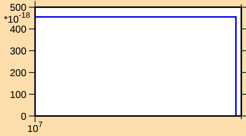
\sigma vs. E for ^{239}\text{Bk} (mt 34)
