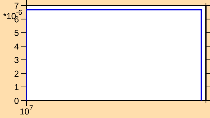
\sigma vs. E for ^{239}\text{Bk}(n,3n)
